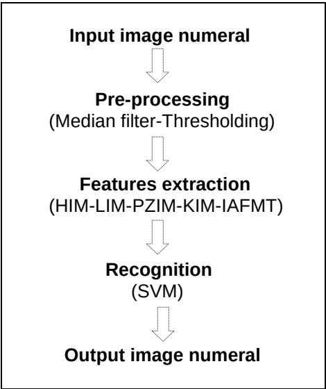
Fig .1. The proposed recognition systems for Eastern Arabic numerals recognition.
