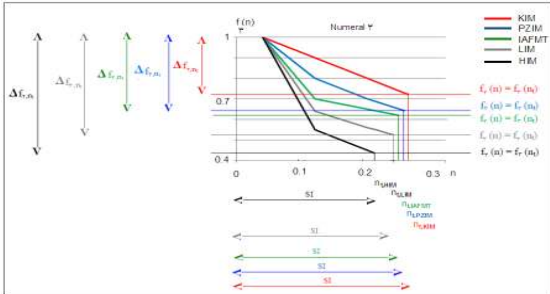
Fig.18.The determination of threshold stability, optimal hyperplane and stability interval of numeral 7 for five moments.
