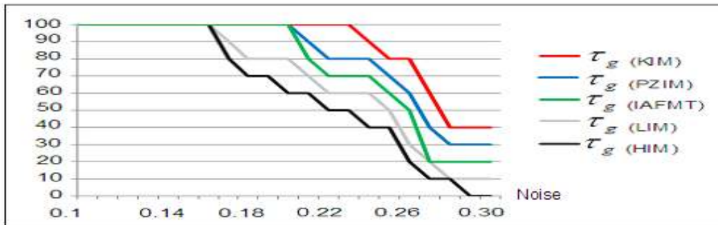
Fig. 7. The graphical representation of global rate recognition in function of noise for each descriptor.
