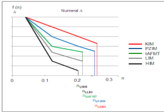
Fig. 16. The variations of decision function f_1 according to added noise to numeral A for five descriptors.
