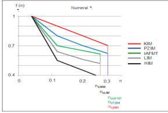
Fig. 14. The variations of decision function f_1 according to added noise to numeral 7 for five descriptors.
