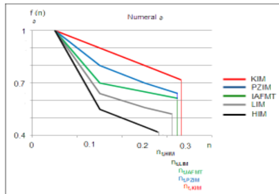
Fig. 13. The variations of decision function f_n according to added noise to numeral 2 for five descriptors.
