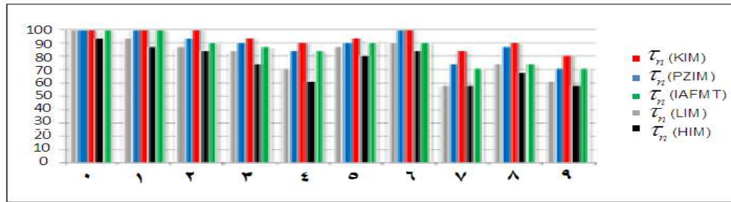
Fig. 5. The graphical representation of recognition rate of each numeral and for each descriptor.
