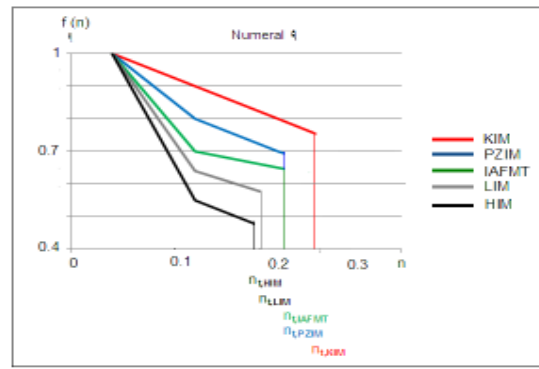
Fig. 17. The variations of decision function f_1 according to added noise to numeral 4 for five descriptors.
