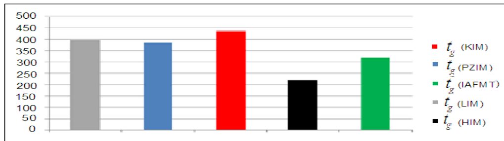
Fig. 6. The graphical representation of global time of execution for each descriptor.
