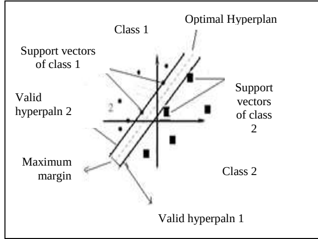
Fig. 3. Linear support vectors machines illustration.
