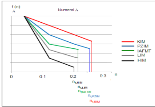
Fig. 16. The variation of decision function f_4 according to added noise to numeral 4 for five descriptors.
