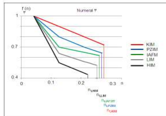
Fig. 11. The variation of decision function f_n according to added noise to numeral 9 for five descriptors.
