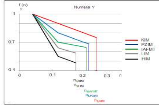
Fig. 15. The variation of decision function f_5 according to added noise to numeral 5 for five descriptors.
