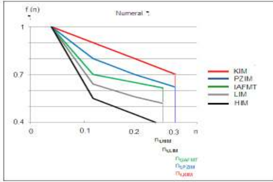
Fig. 14. The variation of decision function f_1 according to added noise to numeral 7 for five descriptors.
