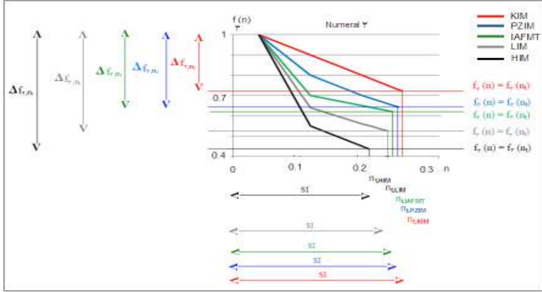
Fig. 18. The determination of threshold stability, optimal hyperplane and stability interval of numeral 7 for five moments.
