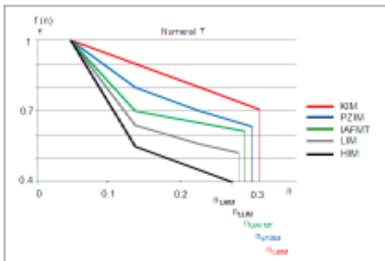
Fig. 10. The variation of decision function f_n according to added noise to numeral 7 for five descriptors.
