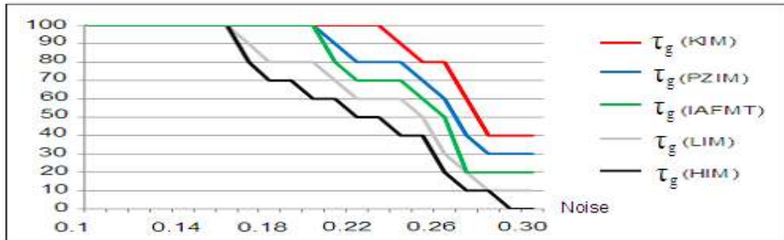
Fig. 7. Graphical representation of global rate recognition depending upon added noise for each descriptor.
