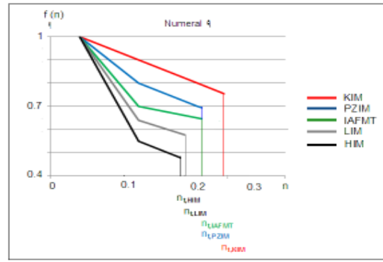
Fig. 17. The variation of decision function f_1 according to added noise to numeral 1 for five descriptors.
