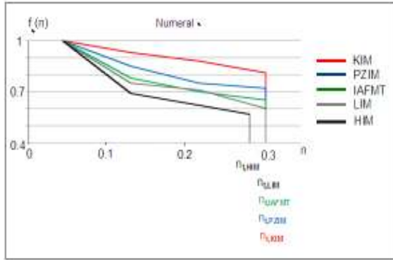
Fig. 8. The variation of decision function f_n according to added noise to numeral 4 for five descriptors.
