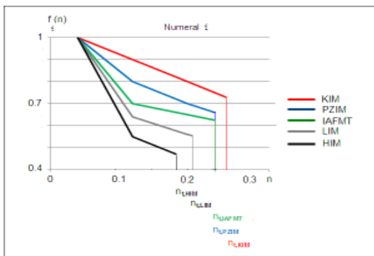
Fig. 12. The variation of decision function f_n according to added noise to numeral 1 for five descriptors.
