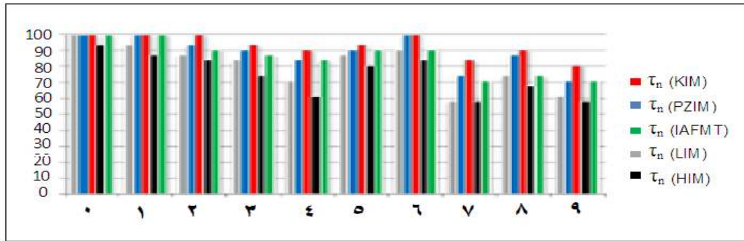
Fig. 5. Graphical representation of recognition rate of each numeral for each descriptor.
