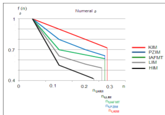
Fig. 13. The variation of decision function f_n according to added noise to numeral 2 for five descriptors.
