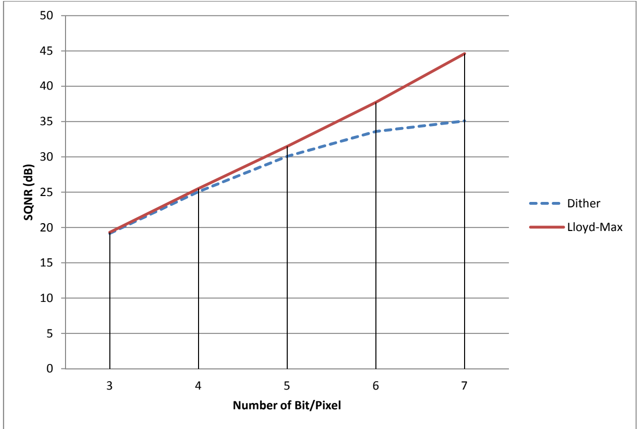
Figure 11.0: Plot of SQNR in decibels (dB) for Dither-based Non-uniform Quantization and Lloyd-Max Non-uniform Quantization Schemes
