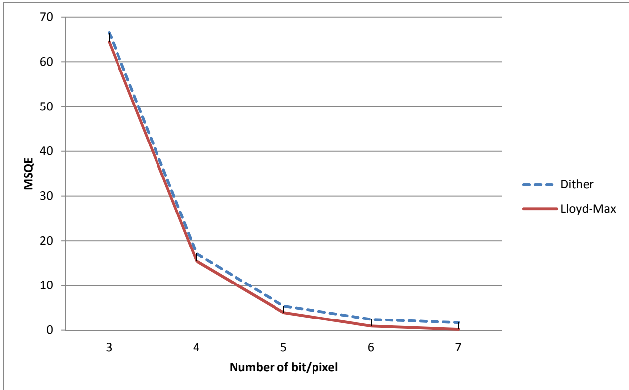
Figure 10.0: Plot of MSQE Values for Dither-based Non-uniform Quantization and Lloyd-Max Non-uniform Quantization Schemes
