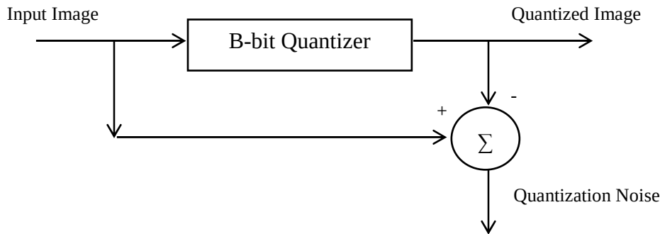
Figure 1.0: Block Diagram of Quantization Process and the Associated Noise
