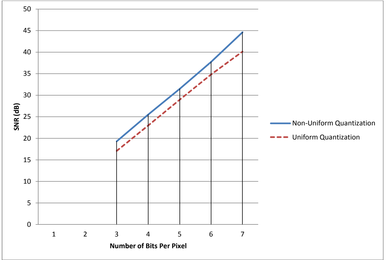
Figure 9.0: Plot of SQNR in decibels (dB) for Non-uniform and Uniform Quantization
