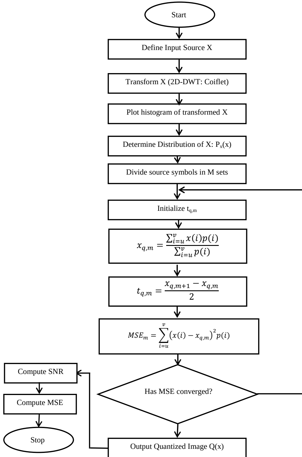
Figure 7.0: Flowchart of the Lloyd-Max Quantization Procedures
