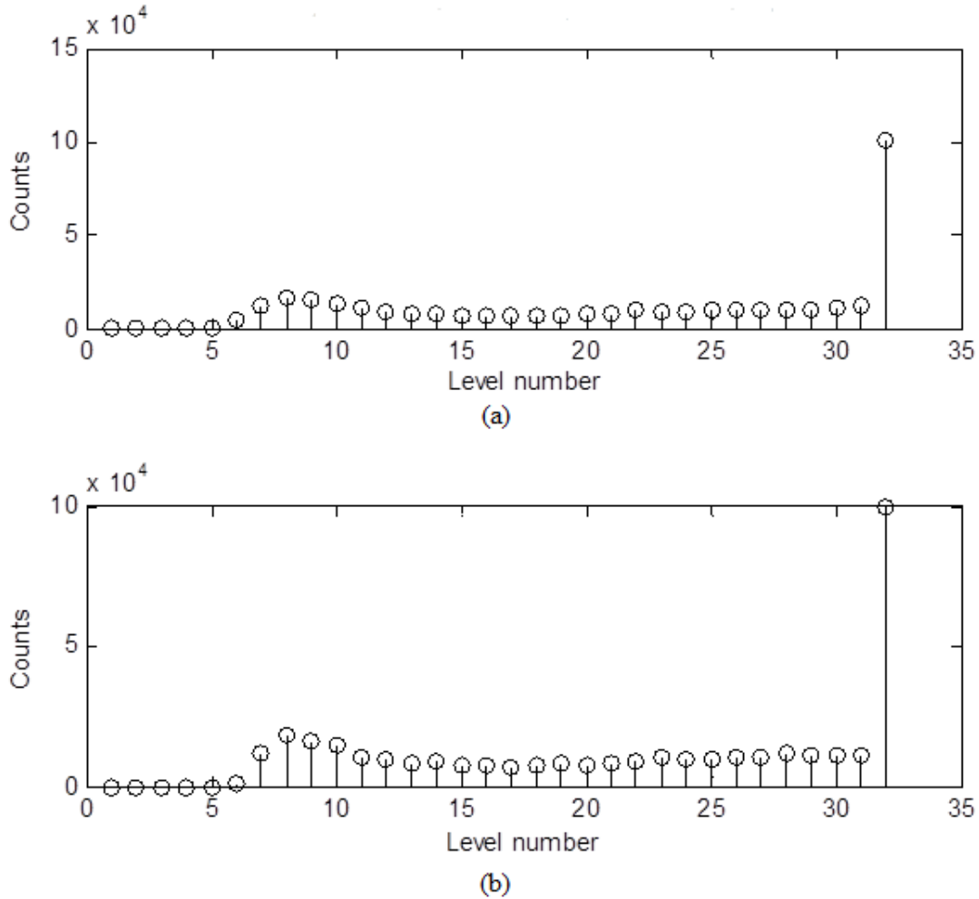
278 Figure 4.0: Histogram Plot of 5 bpp Quantized Fingerprint Output (a) and 8 bpp Source 279 fingerprint Input (b)
