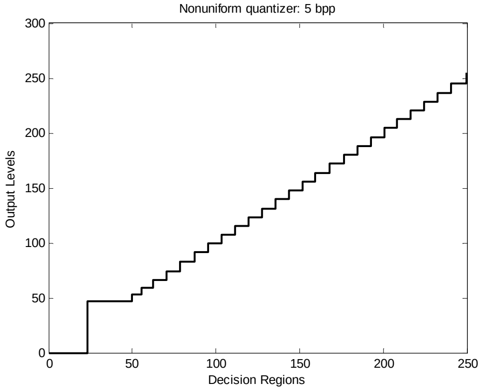
Figure 6.0: Plot of the Non-uniform Quantization Output Levels at 5 bpp
