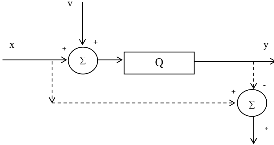
Figure 3.0: The Non-subtractive dithered quantization schematic.
