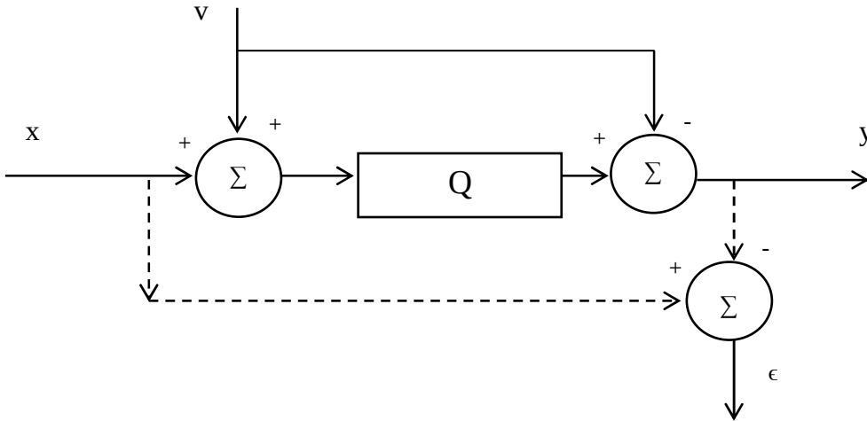
Figure 2.0: The Subtractive Dithered Quantization Schematic.
