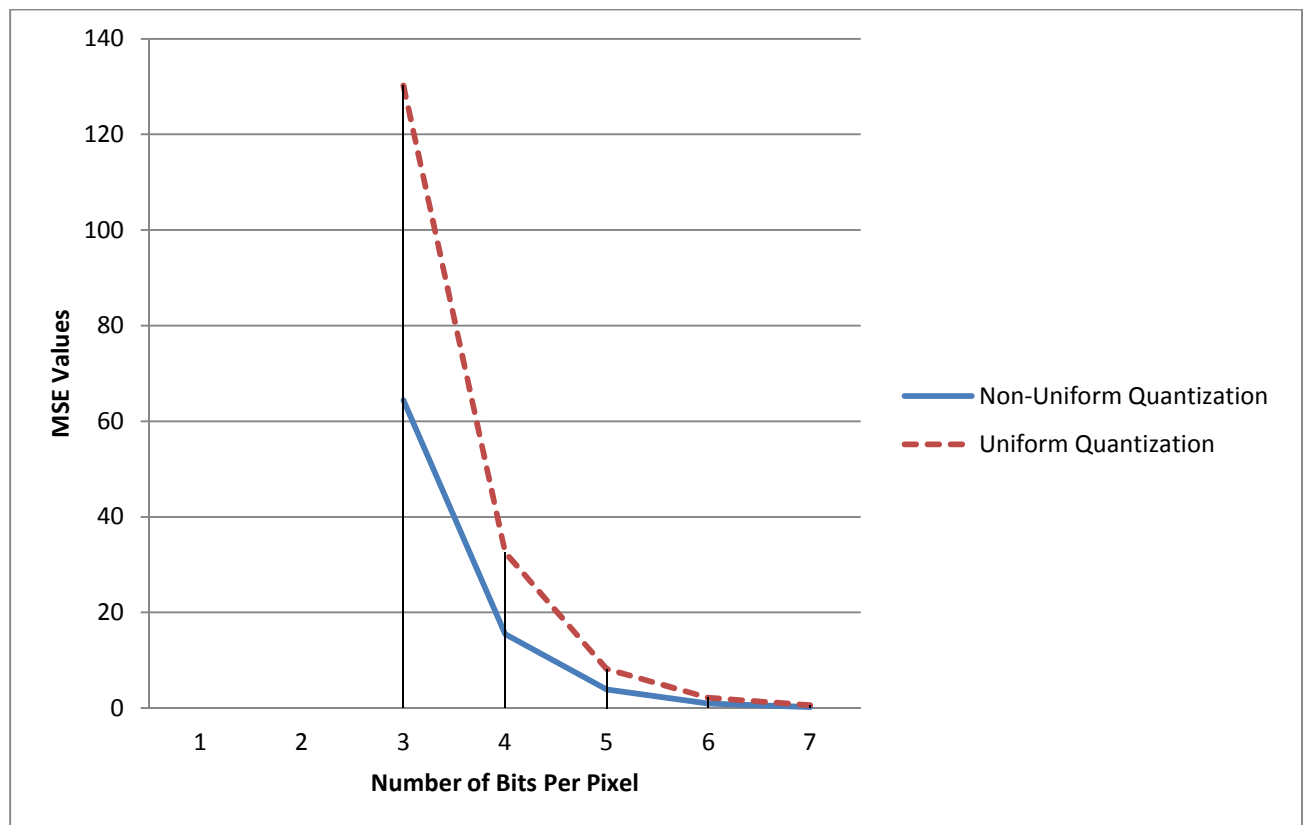
Figure 8.0: Plot of MSQE Values for Non-uniform and Uniform Quantization
