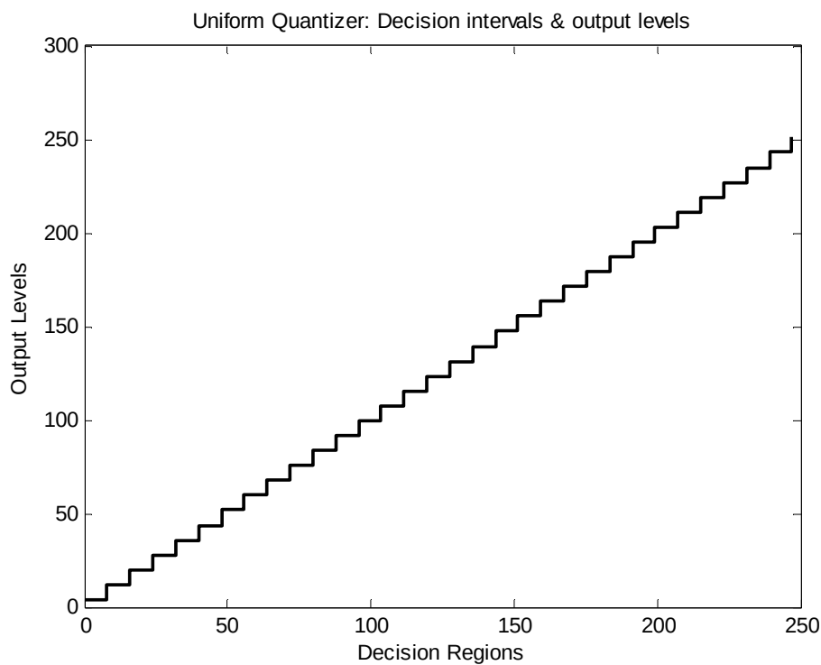
Figure 5.0: Plot of the Uniform Quantization Output Levels at 5 bpp
