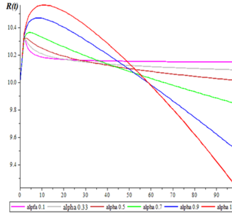
Figure 1: Calculated curves the aerosol radius, constructed according to the decision (2.7) of the generalized model LSW depending on the parameter values \alpha
