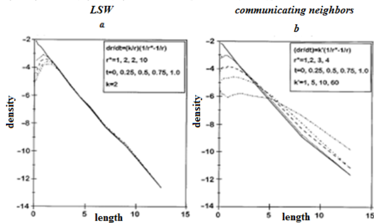
Figure 2: The calculated curves of the radius of crystals, presented in [Michael (1998)] a – classical theory LSW; b - the theory of "communicating neighbors"
