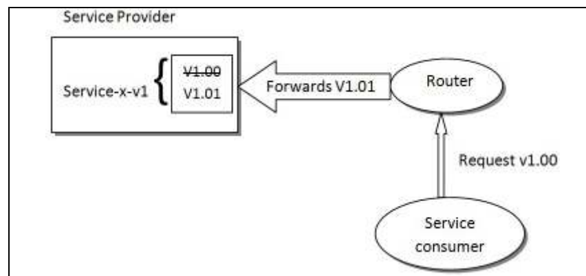
Figure 8: Non-functional of Non-breaking change
