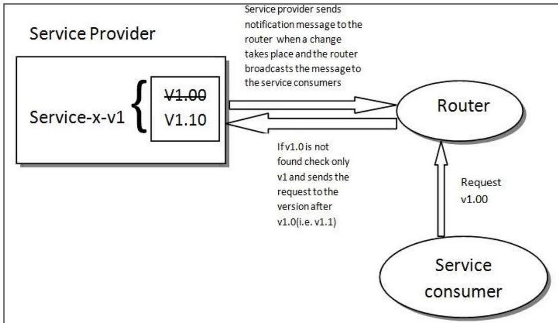
Figure 9: Non-breaking Functional change
