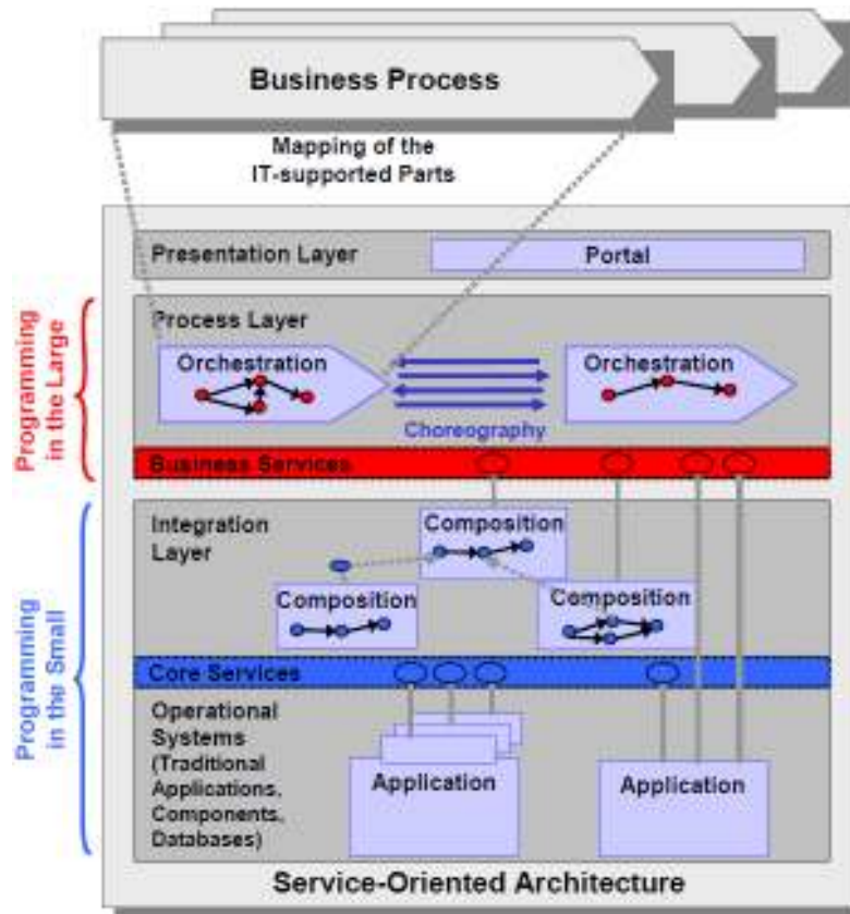
Figure-1- SOA layers
