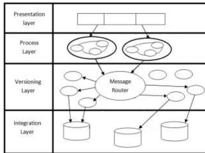
Figure -2- New Structure of SOA layers
