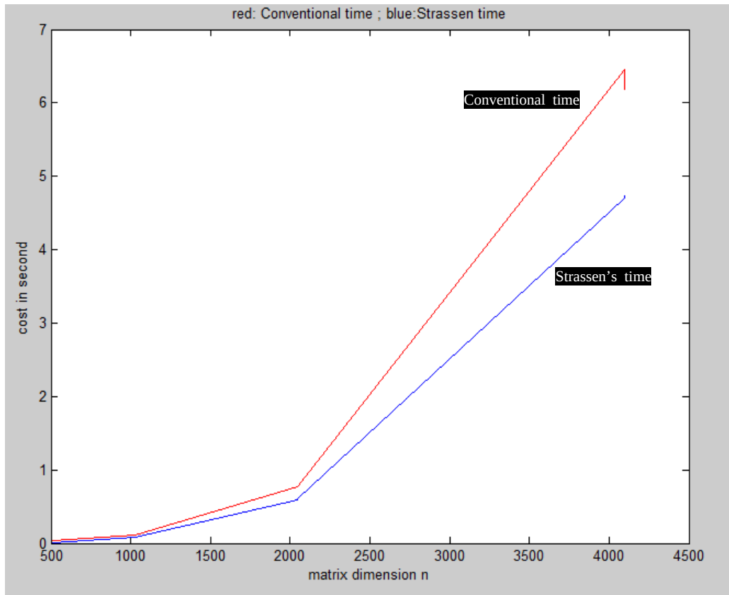
Figure 4.3: graph of experiment with three recursions
