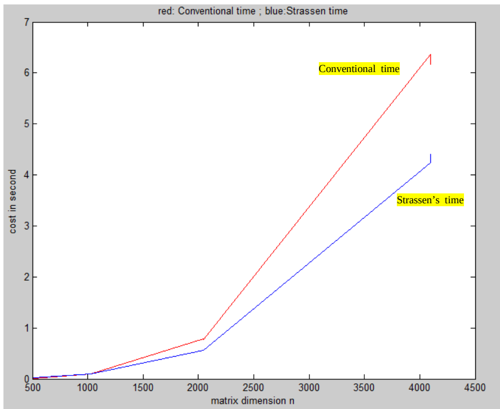
Figure 4.2: graph of experiment with four recursions
