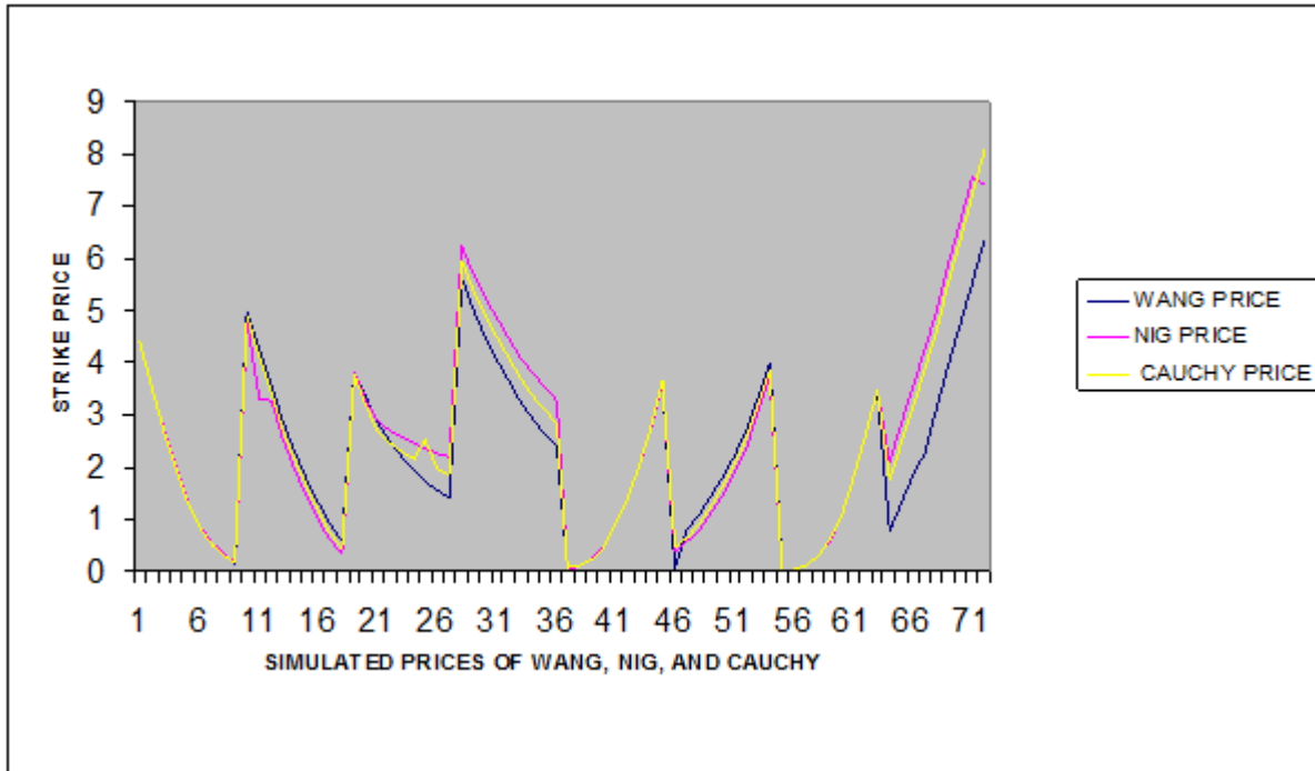
Figure 1.0: The graph of Strike price against Wang, NIG and Cauchy Prices
