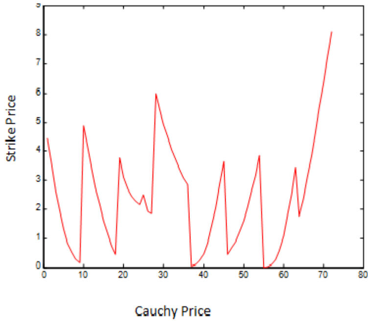
Figure 3: The graph of Strike Price against Cauchy Price.
