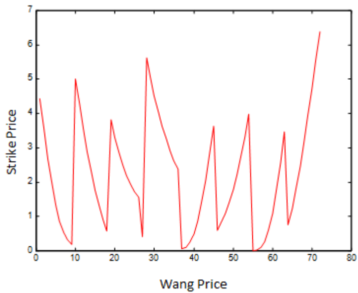
Figure 1: The graph of Strike Price against Wang Price
