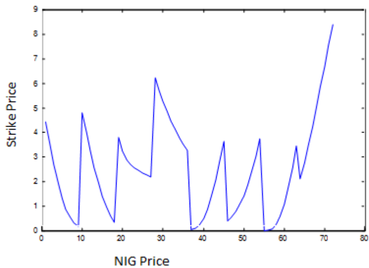
Figure 2: The graph of strike Price against NIG Price
