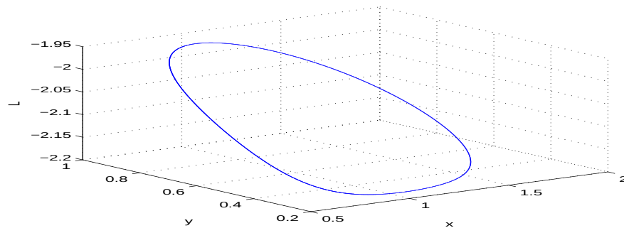
Fig. 9. The profile of L(x, y) for a = 0.5 , b = c = d = 1 and initial conditions (x_0 = 0.5, y_0 = 0.5) and (x_0 = 0.95, y_0 = 0.95) respectively.
