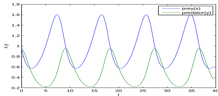
Fig. 2. Profile of the numerical solution (x(t), y(t)) , for a = 0.5, b = c = d = 1 and initial conditions (x_0 = 0.5, y_0 = 0.5) , (x_0 = 0.95, y_0 = 0.95)
