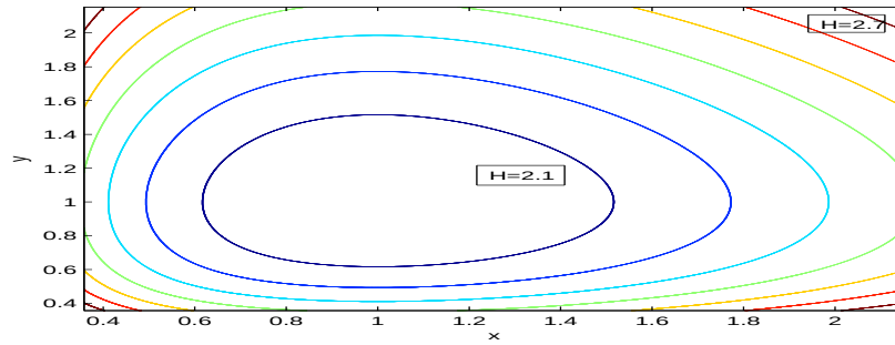
Fig. 6. The profile of H(x, y) for a = 0.5 , b = c = d = 1 and initial conditions (x_0 = 0.5, y_0 = 0.5) , and (x_0 = 0.95, y_0 = 0.95) respectively.
