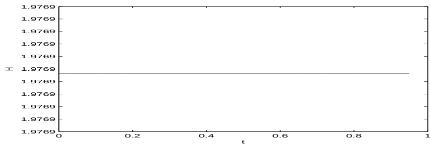
Fig. 5. The profile of the Hamiltonian H as function of t , for a = 0.5 , b = c = d = 1 and initial conditions (x_0 = 0.5, y_0 = 0.5) , and (x_0 = 0.95, y_0 = 0.95) respectively.
