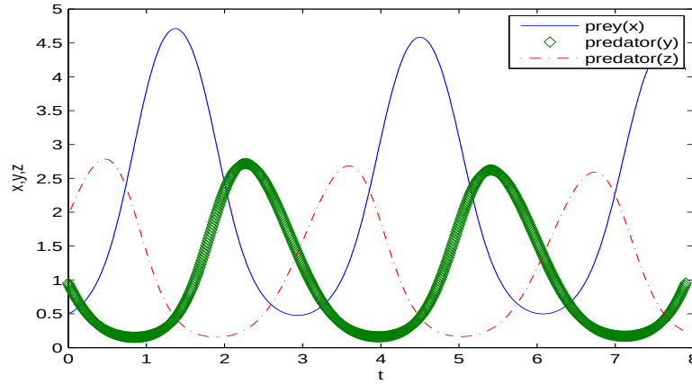
169 Fig. 10. The profile of the numerical solution (x(t), y(t), z(t)) , for the initial conditions (x_0 = 0.5, y_0 = 1, z_0 = 2) .
