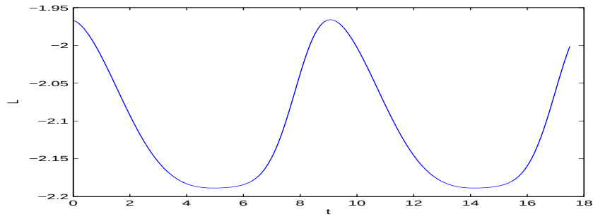
Fig. 8. The profile of the Lagrangian L as function of t for a = 0.5 , b = c = d = 1 and initial conditions (x_0 = 0.5, y_0 = 0.5) , and (x_0 = 0.95, y_0 = 0.95) respectively.
