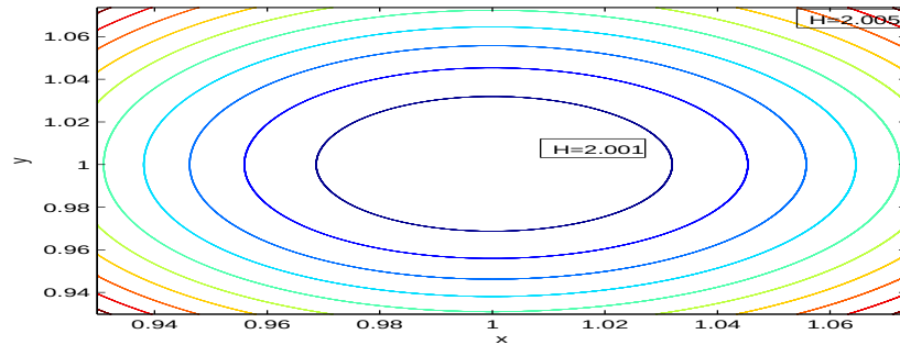
Fig. 7. Some level curves of H(x, y) for a = b = c = d = 1 and initial conditions (x_0 = 0.5, y_0 = 0.5) , and (x_0 = 0.95, y_0 = 0.95) respectively.
