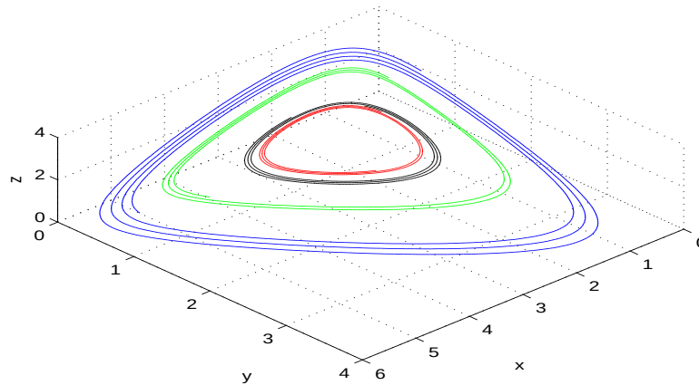
171 Fig. 11. Phase space portrait for the initial conditions (x_0 = 0.5, y_0 = 0.95, z_0 = 2.95) , (x_0 = 0.5, y_0 = 0.5), z_0 = 172 1.95) , (x_0 = 1, y_0 = 0.75, z_0 = 1.25) , (x_0 = 2.1, y_0 = 0.35, z_0 = 1.55) listed in order from outermost trajectory to 173 innermost trajectory.
