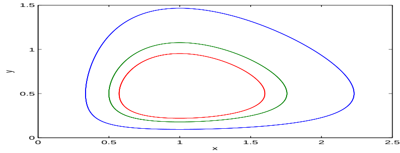
Fig. 3. Phase space portrait for a = 0.5 , b = c = d = 1 and initial conditions (x_0 = 0.35, y_0 = 0.35) , (x_0 = 0.5, y_0 = 0.5) , (x_0 = 0.95, y_0 = 0.95) listed in order from outermost trajectory to innermost trajectory.
