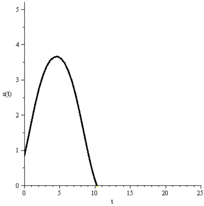
Fig.6. The case i of initial conditions, t=0..25
