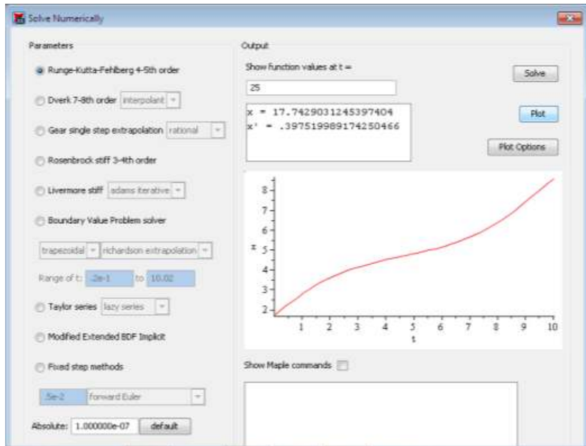
Fig.5 The case ii of solution analysis
