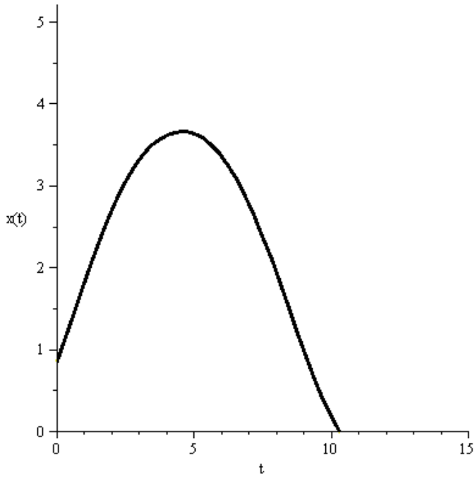
Fig.8. The case i, t=0..15
