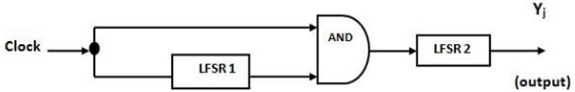
Figure 21: clock control
