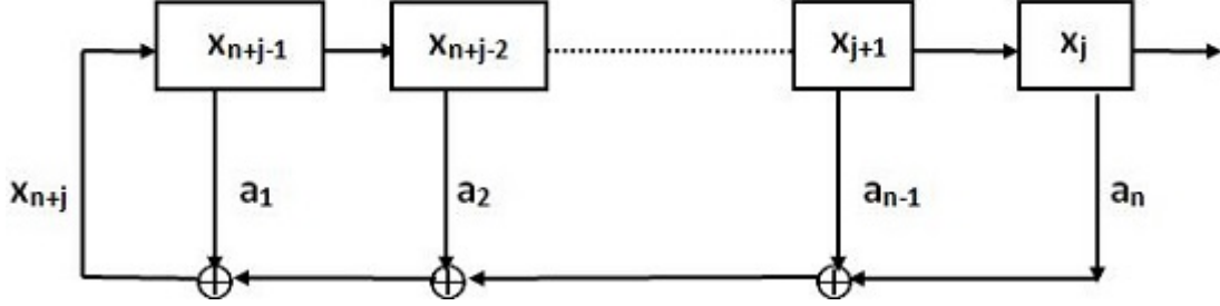
Figure 4: A scheme of LFSR
