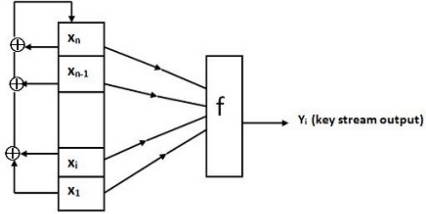
Figure 20: Non linear filter generator
