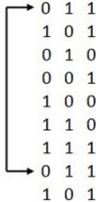
Figure 8: 3-bits LFSR
