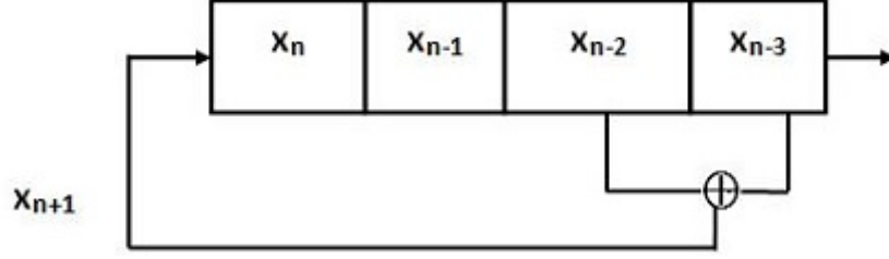
Figure 16: 4-bits LFSR
