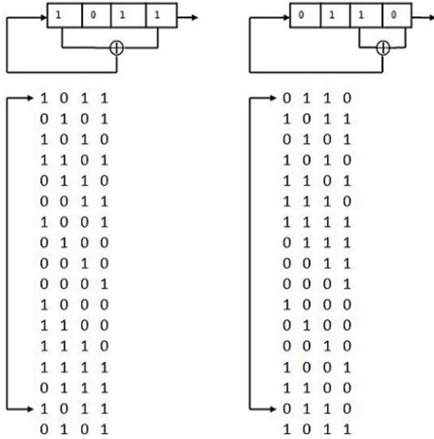
Figure 11: 4-bits LFSR
