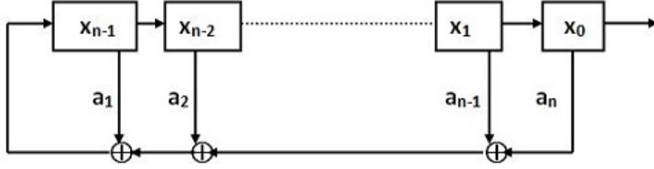
Figure 5: LFSR in mode Fibonacci
