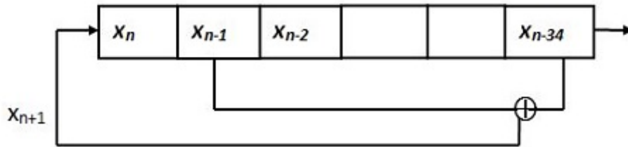
Figure 17: 35 bits LFSR
