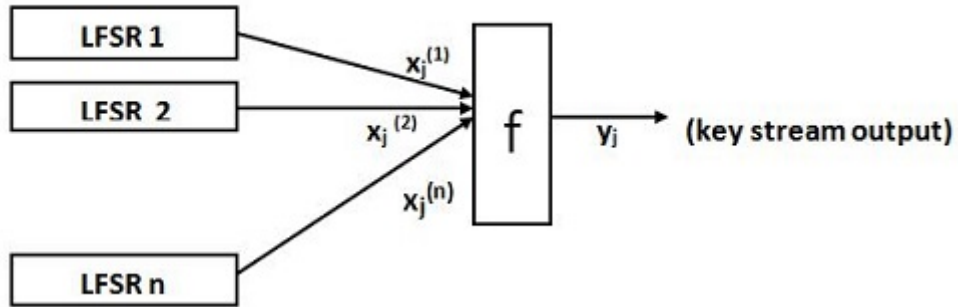
Figure 19: Non linear combined LFSRs
