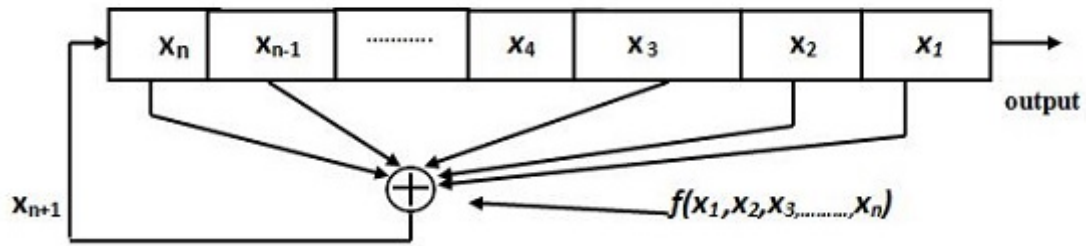
Figure 7: n-bits LFSR
