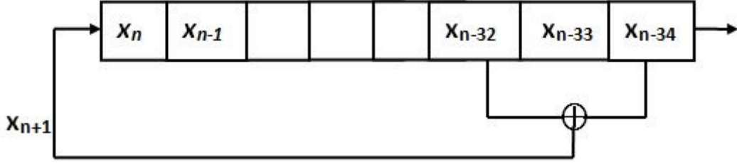
Figure 18: 35 bits LFSR
