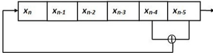
Figure 12: 6-bits LFSR
