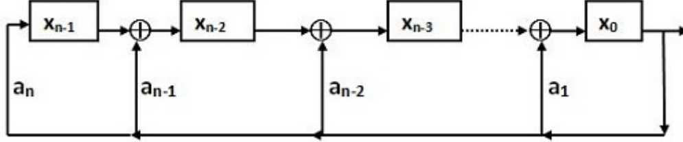
Figure 6: LFSR in mode Galois
