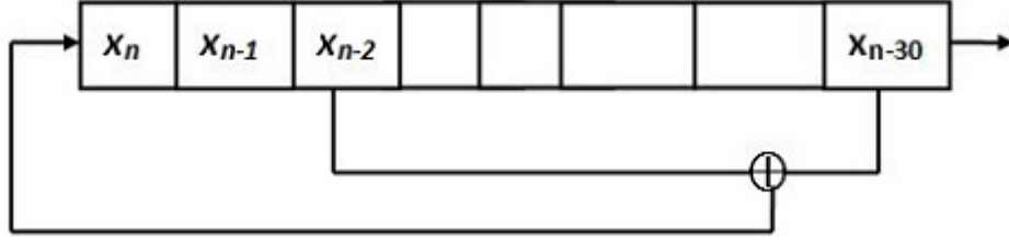
Figure 13: 31-bits LFSR
