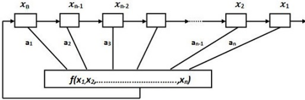
Figure 3: General Scheme of Linear Feedback Shift Register
