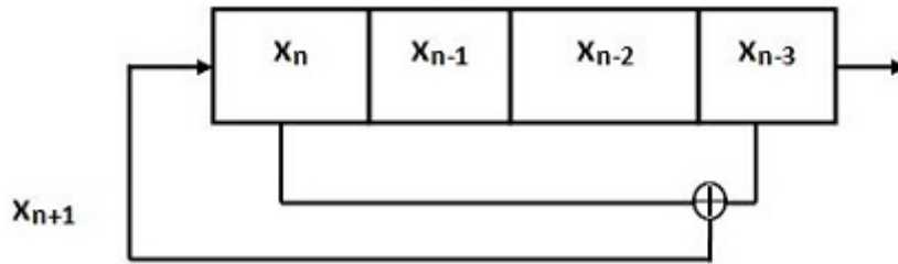
Figure 15: 4 bits LFSR
