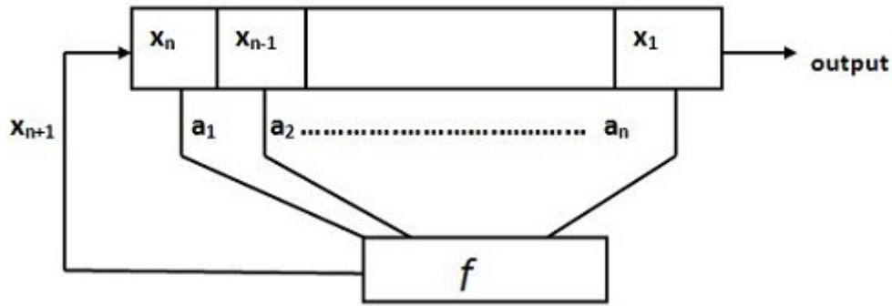
Figure 14: n -bits LFSR
