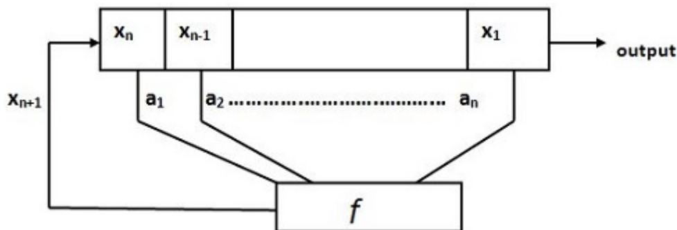
Figure 14: n-bits LFSR
