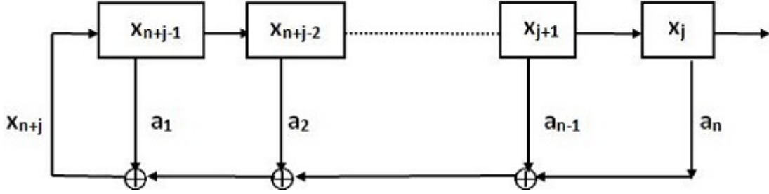
Figure 4: A scheme of LFSR
