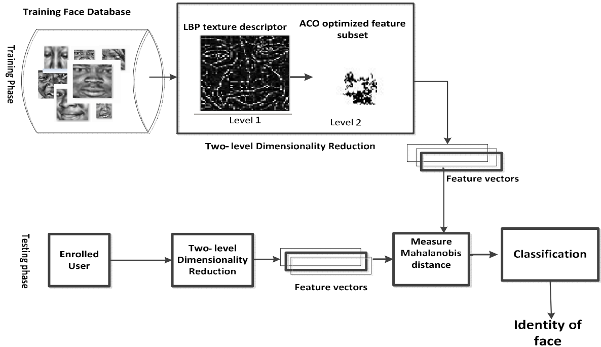
Figure 1: Process flow of the Feature Dimensionality Reduction Technique for Face Recognition System
