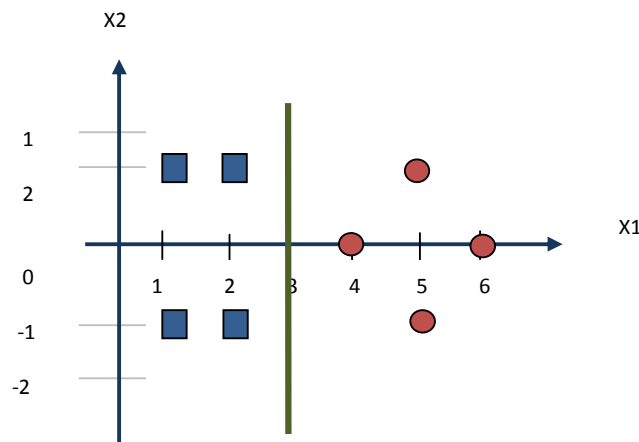
Fig 5: Decision plane with optimum decision boundary
