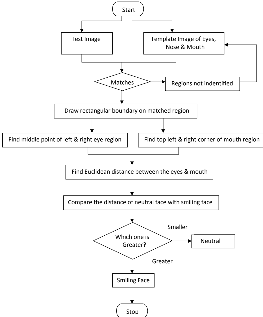
Fig 1: Overall processing of neutral or smiling face detection
