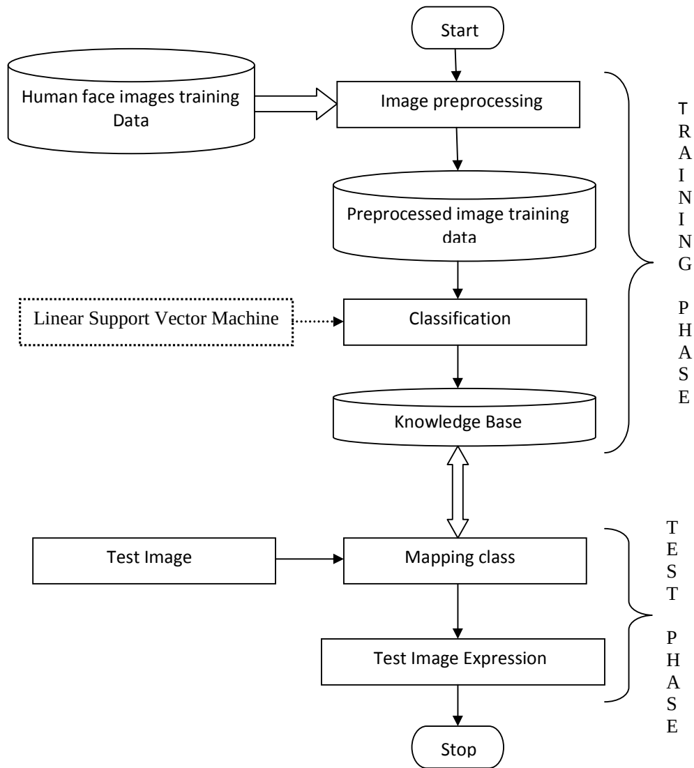
Fig 2: Overall processing of expression classification
