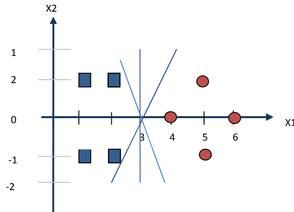
Fig 3: Decision plane in SVM
