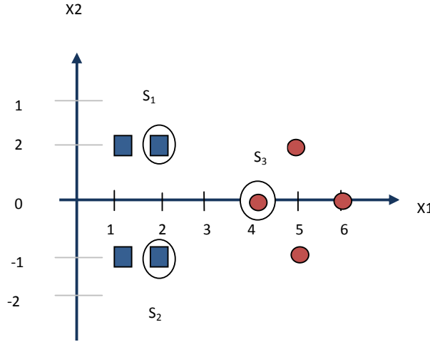
Fig 4: Support vectors used in SVM classification
