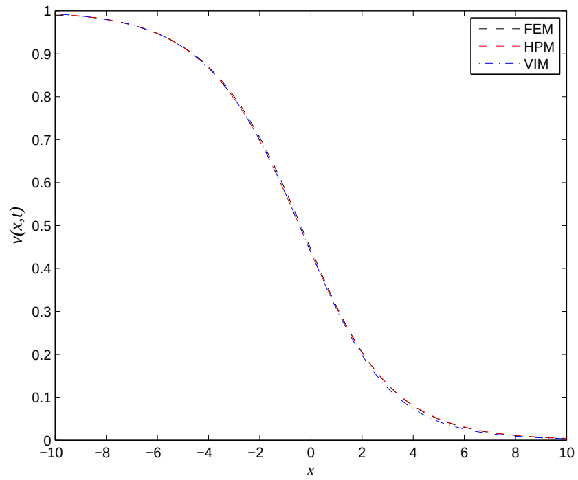
Figure 2: Comparison between the traveling wave solution of v(x, t) using VIM, HPM and COMSOL, when t = 0.5 .
