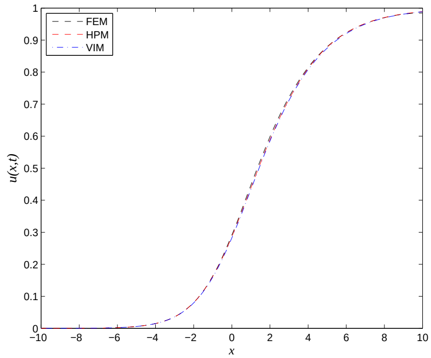
Figure 1: Comparison between the traveling wave solution of u(x, t) using VIM, HPM and COMSOL, when t = 0.5 .
