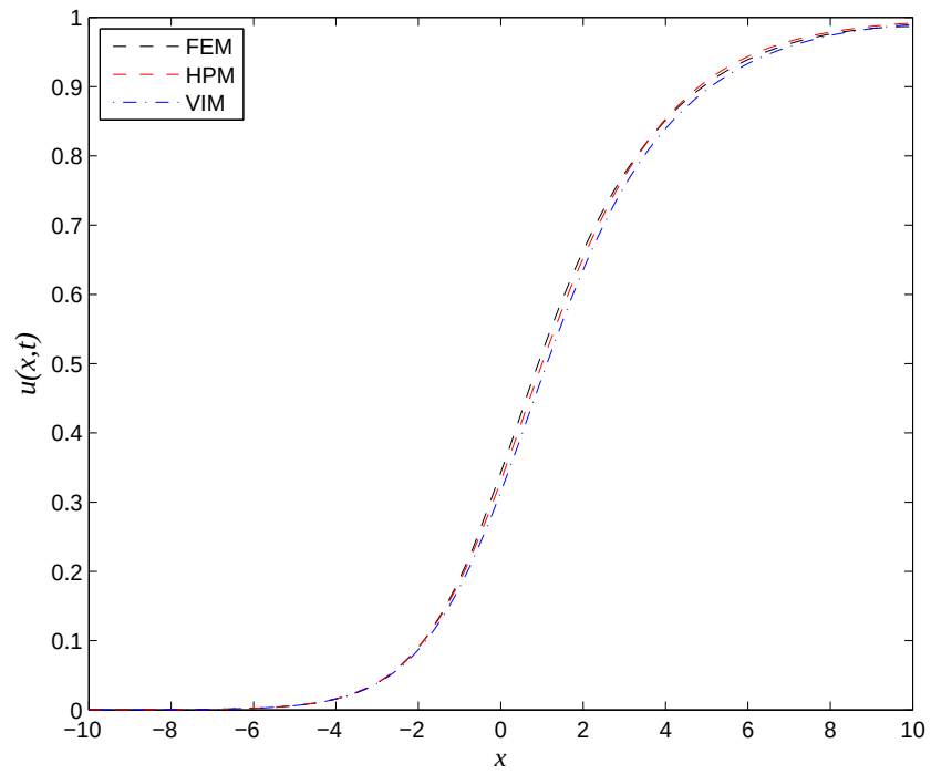
Figure 3: Comparison between the traveling wave solution of u(x, t) , using VIM, HPM and COMSOL, when t = 1 .
