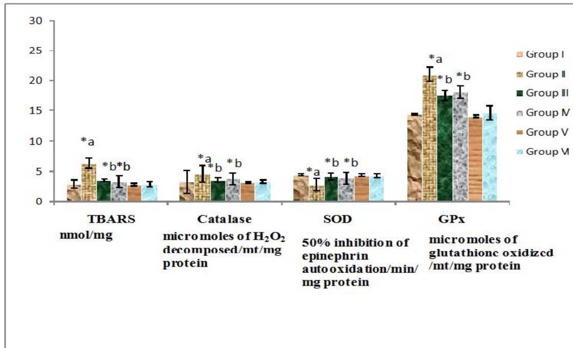
Figure 2- Effect of NAT-L and NAT-S extract on the antioxidant activity in normal and experimental rats. Values are expressed as mean \pm S.D. for six animals. Comparisons are made between: *a, Group I vs. Groups II; *b, Group II vs. Groups III and IV. The letters *a and *b represent the Statistical significance at p < 0.05 .
