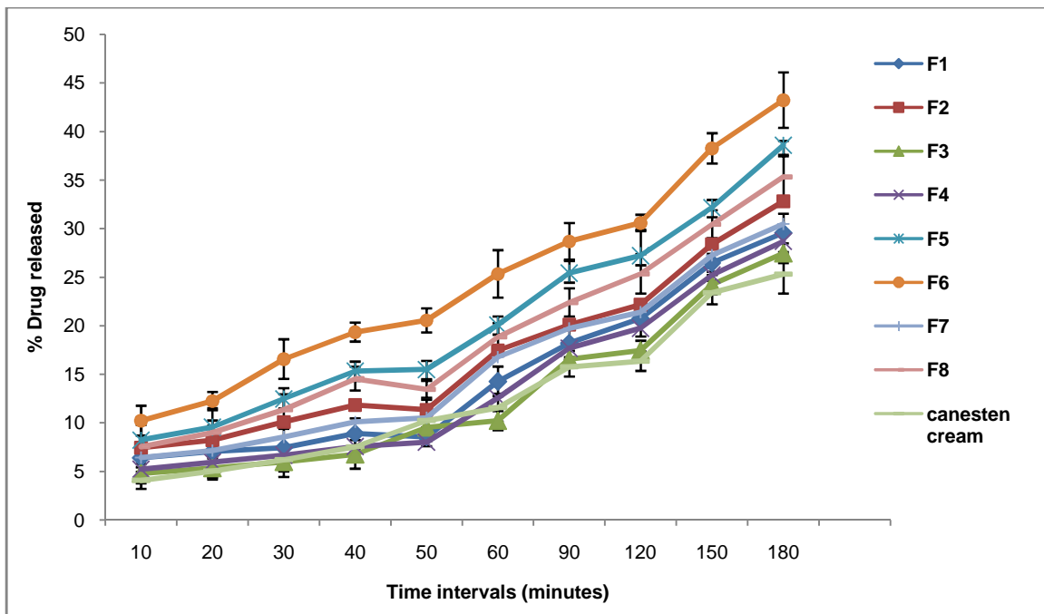
Fig.6. Release profiles of Clotrimazole from its emulgel formulations.
