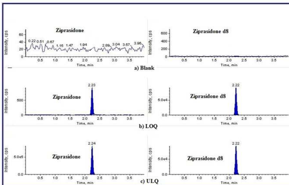
Fig.3. Chromatogram of a) Blank b) LOQ c) ULQ of Ziprasidone and Ziprasidone d8
