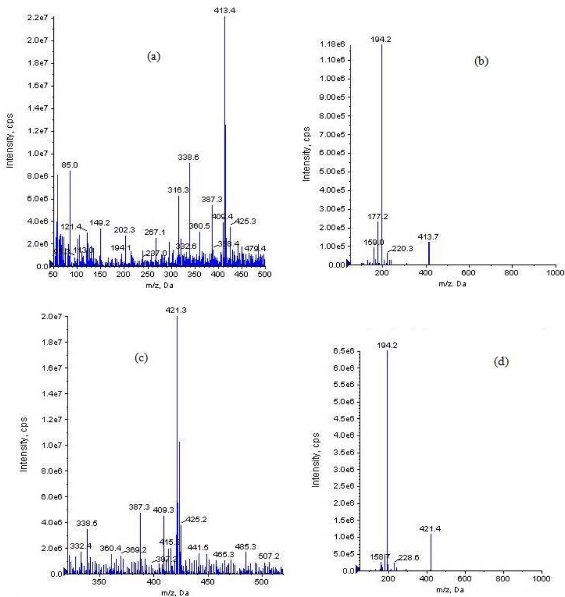
Fig.2. Mass spectrum of (a) Ziprasidone Parent ion, (b) Ziprasidone Product ion,
