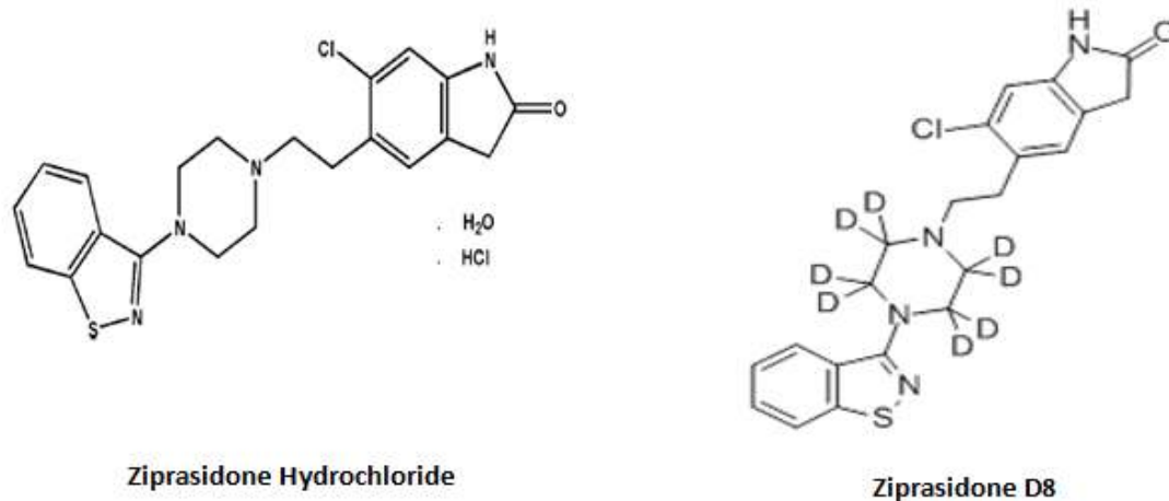
Fig.1. Chemical Structures of Ziprasidone and Ziprasidone D8
