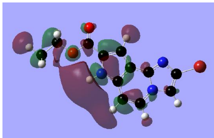
Figure 13. Localization of the local (LUMO+1)* of atom 9 in molecule 2 (isovalue = 0.02).
