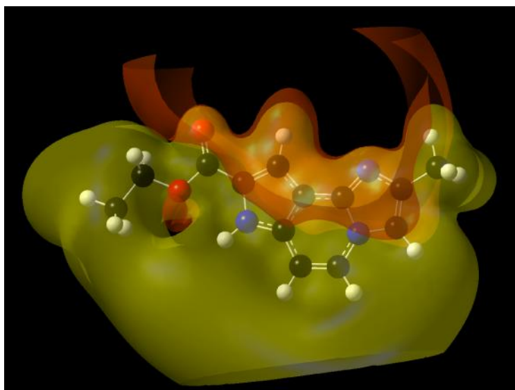
Figure 5. Molecular electrostatic potential of molecule 3. The orange isovalue surface corresponds to negative MEP values (-0.01) and the yellow isovalue surface to positive MEP values (0.01).
