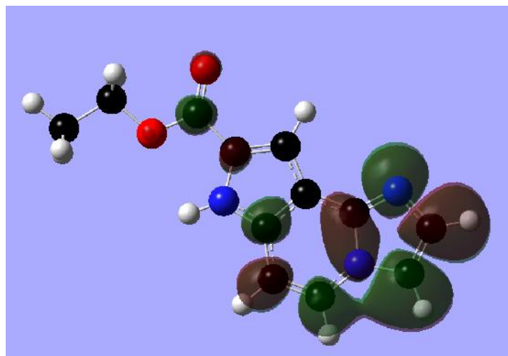
Figure 12. Localization of the local (LUMO+1)* of atom 9 in molecule 1 (isovalue = 0.02).
