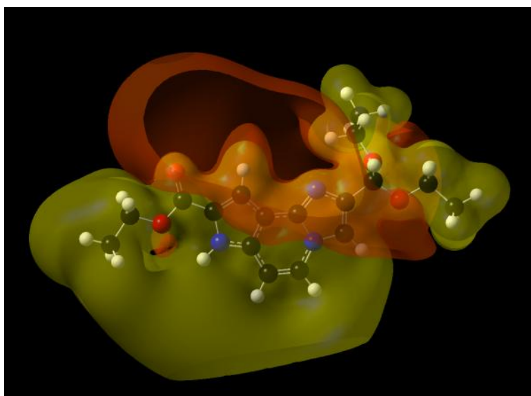
Figure 4. Molecular electrostatic potential of molecule 12. The orange isovalue surface corresponds to negative MEP values ( -0.01 ) and the yellow isovalue surface to positive MEP values ( 0.01 ).
