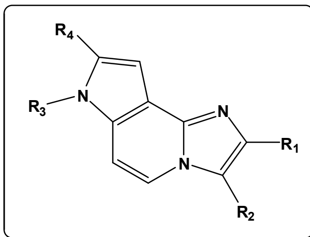
Figure 1. Imidazo[1,2- a ]pyrrolo[2,3- c ]pyridine derivatives.
