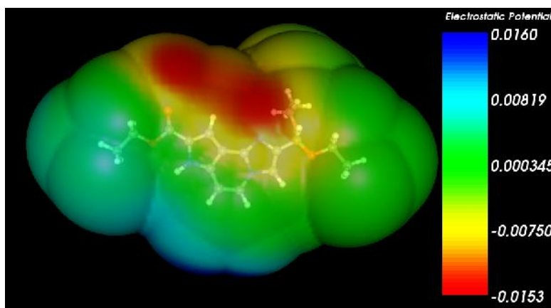
Figure 6. Molecular electrostatic potential of molecule 12 at a distance of 3.5 Å from the nuclei.
