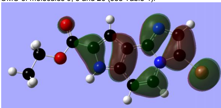
220 221 Figure 8. Localization of the highest occupied molecular orbital (HOMO) of molecule 9 (isoval = 0.02).
