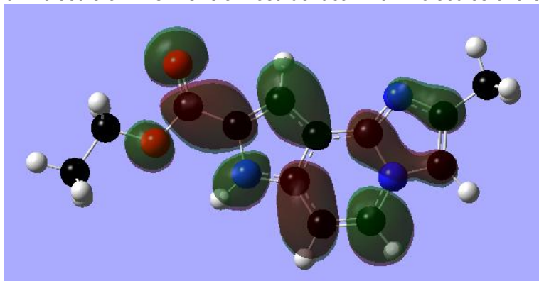
Figure 11. Localization of the lowest vacant molecular orbital (LUMO) of molecule 3 (isovalue = 0.02). The magnitude of the localization and the nature of the local MOs can be very different. For example Figs. 12 to 14 show, respectively, the local (LUMO+1)* of atom 9 (see Fig. 2) of molecules 1, 2 and 13.
