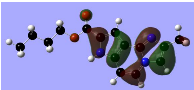
Figure 10. Localization of the highest occupied molecular orbital (HOMO) of molecule 26 (isovalue = 0.02). We can see that the HOMO is of \pi nature in all molecules and localized on rings A, B and C. The substituents alter the localization of the HOMO on specific atoms. Note, for example, that the HOMO is not localized on atom 8 (See Fig. 2) in molecule 9, while it is in the case of molecule 5. These differences in the localization of a frontier MO should provide the basis for a fine explanation of, for example, a \pi - \pi stacking interaction and/or the electron donating properties of a given atom.
