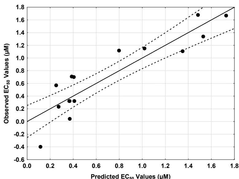
Figure 3: Observed versus calculated values (Eq. 4) of \log(EC_{50}) . Dashed lines denote the 95% confidence interval.
