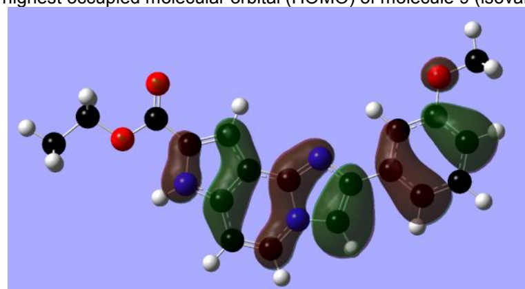
222 223 Figure 9. Localization of the highest occupied molecular orbital (HOMO) of molecule 5 (isoval = 0.02).
