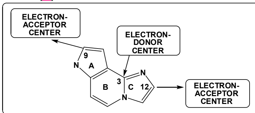
205 206 Figure 8. Partial 2D antiviral pharmacophore. 207
