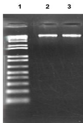
Figure. 1. Metagenomic DNA extracted with the improved method developed in this study: 1, 1 Kb DNA Ladder; 2, DNA from Ch IIs; 3, DNA from Ch IId.
