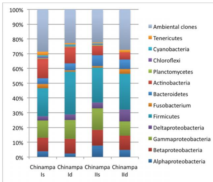
Figure 2. Community composition of bacteria and relative abundance of different bacteria groups estimated from the T-RFLP analysis in the chinampa soils. Ch Is, Ch Id, Ch IIs, and Ch IId represent soil sampled from chinampa I (0-30 cm), chinampa I (30-60 cm), chinampa II (0-30 cm), and chinampa II (30-60 cm), respectively.
