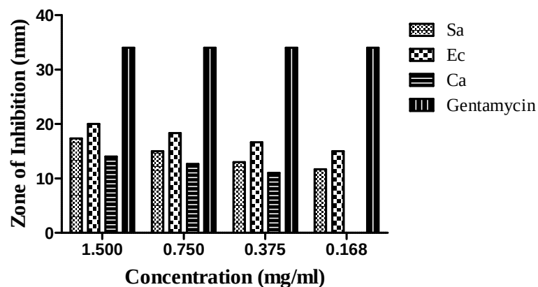
Fig. 1: Comparative Inhibitions of Crude extract of P.tomentosa plant against S. aureus , E.coli , and Candida with gentamycin.
