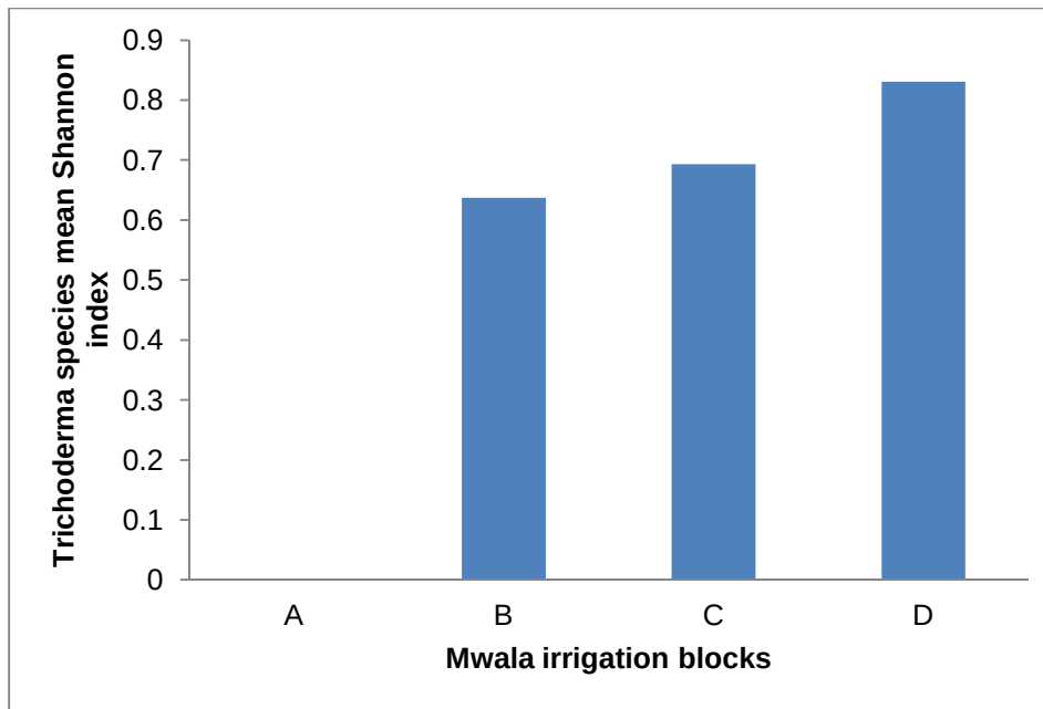
Figure 10: Trichoderma species mean Shannon indices for the four Mwala irrigation blocks.
