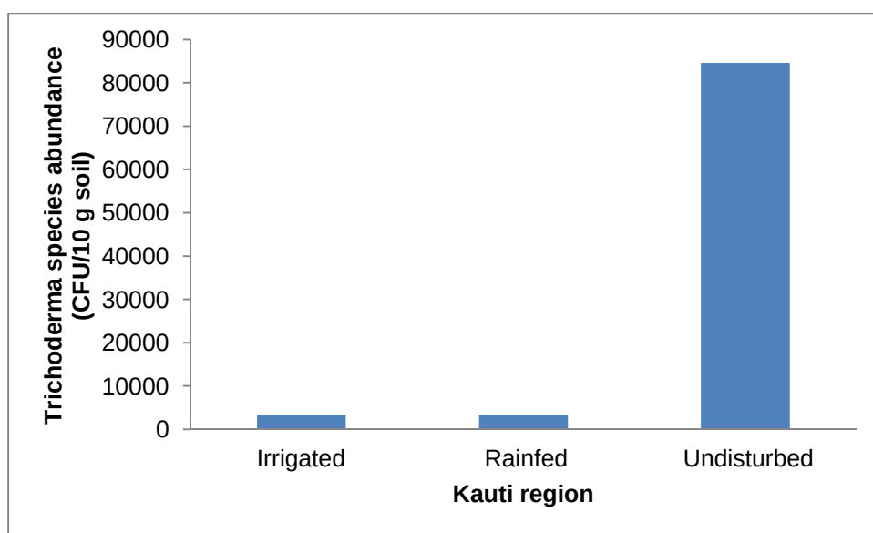
Figure 5: Trichoderma species mean abundance in the three land-use types within Kauti region
