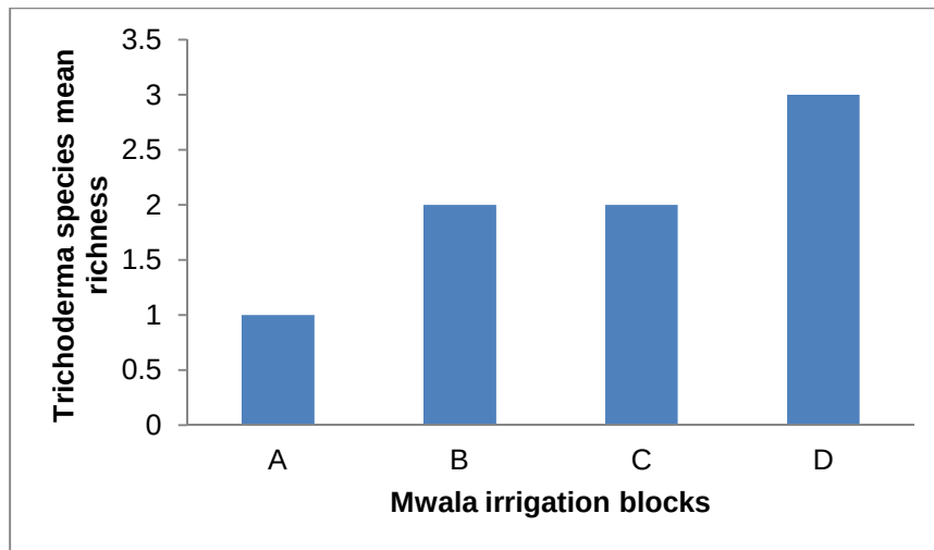
Figure 8: Trichoderma species richness within Mwala irrigation blocks.
