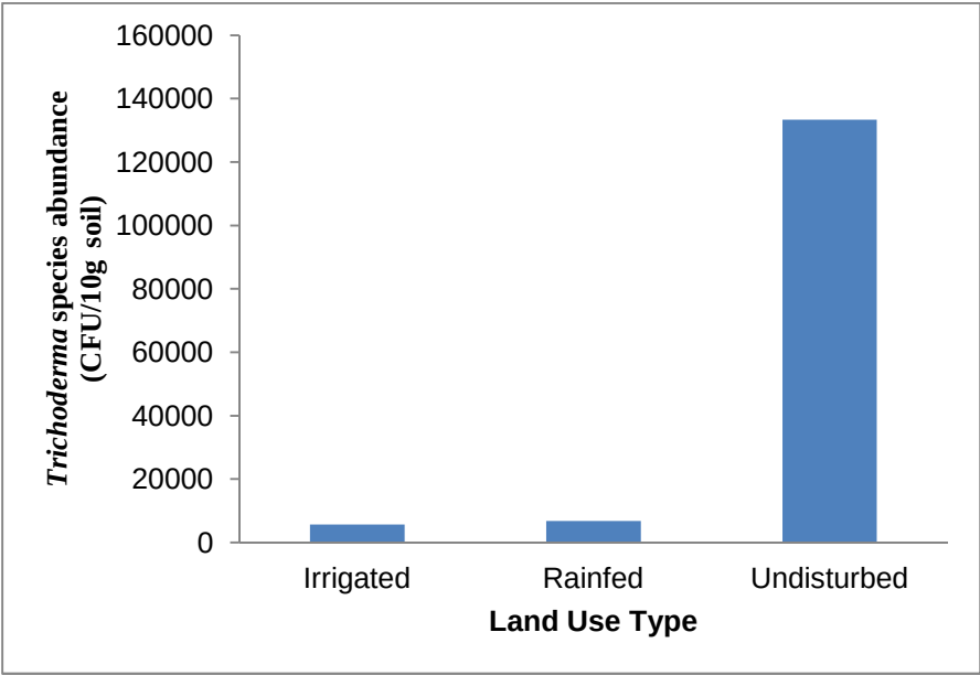
Figure 3: Trichoderma species mean abundance for the three land-use types.
