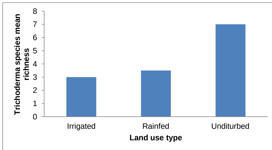
Figure 7: Trichoderma species richness for the three land use types.
