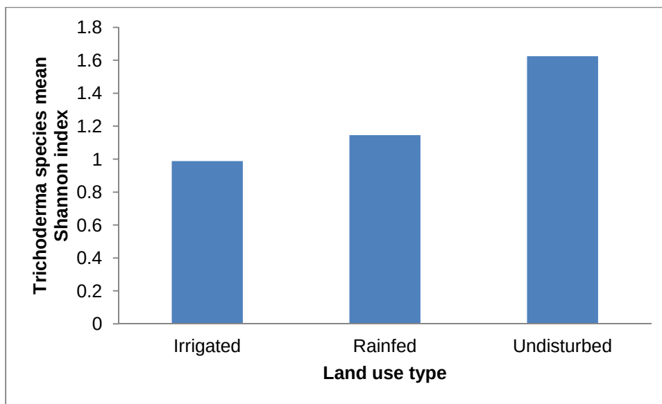
Figure 9: The diversity of Trichoderma species in the three land-use types.
