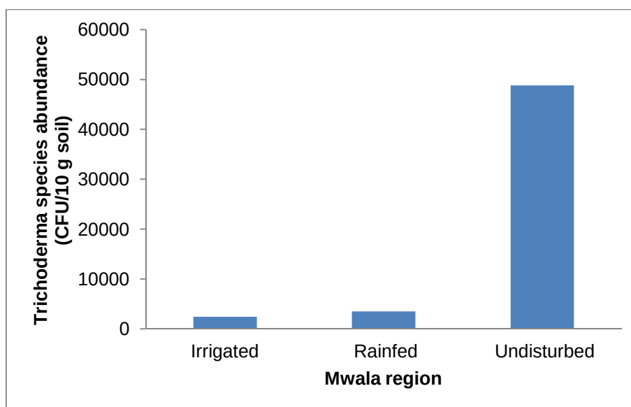
Figure 4: Trichoderma species mean abundance in three land-use types within Mwala region.
