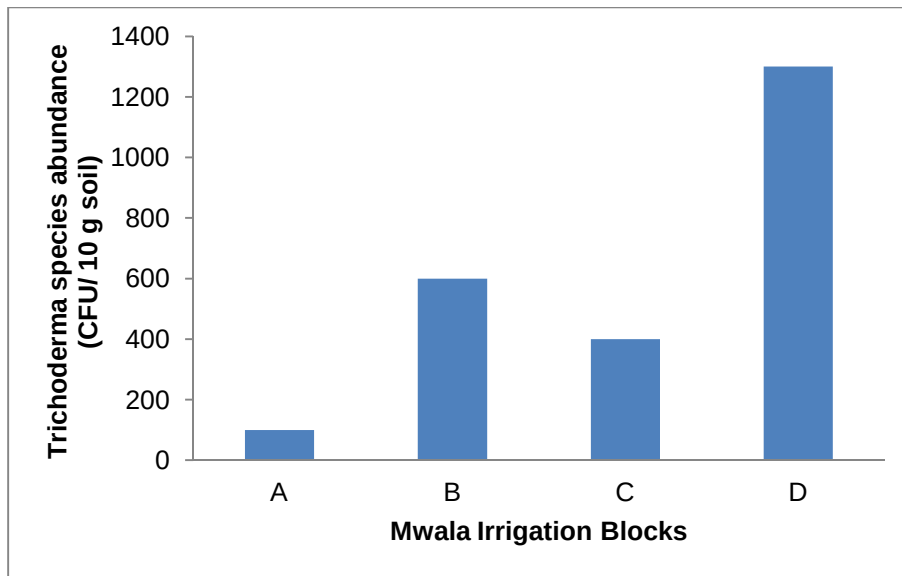
Figure 6: Trichoderma species mean abundance in the four irrigation blocks in Mwala region.
