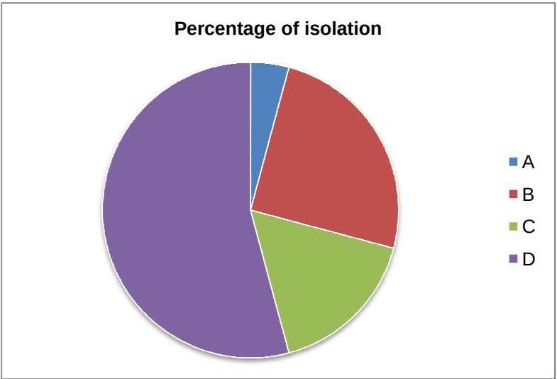
Figure 2: Frequency of isolation of Trichoderma species in Mwala irrigation blocks A to D.
