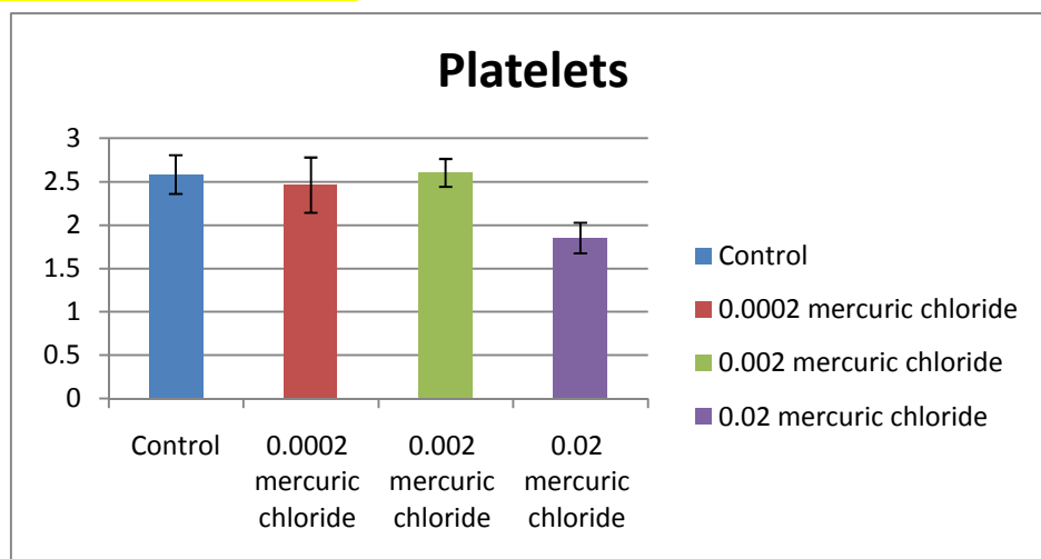
Fig.4. Changes in platelets number ( \times 10^5 \text{ cells/mm}^3 ) in all experimental groups.
