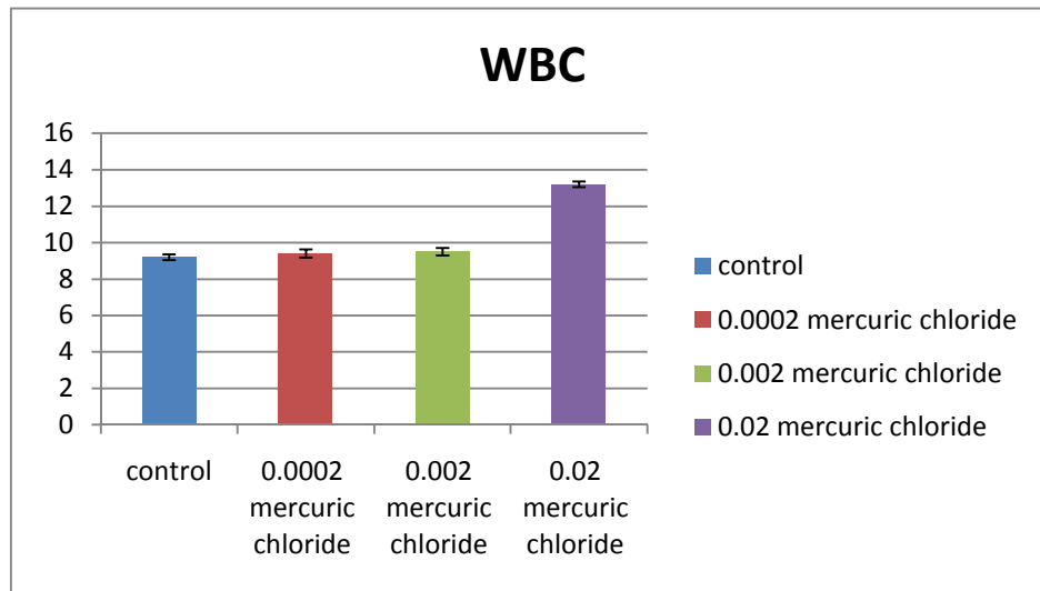
Fig.6: Differences in WBCs count ( \times 10^3 cells/mm 3 ) in all experimental groups.
