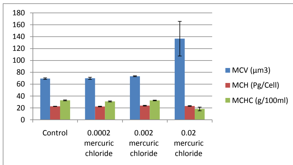
Fig.3. Changes in MCV, MCH and MCHC values in all experimental groups.
