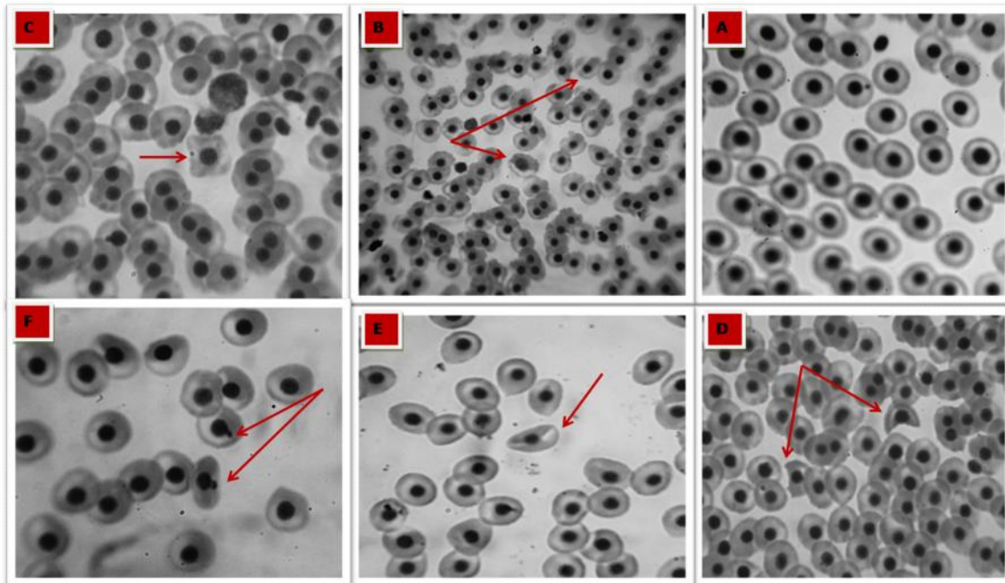
Fig.5. Blood smear for morphological anomalies.[A] showing normal RBC morphology of the control group , while [B] showing fragmented, crenated and enlarged RBC with giant nucleus , [C] showing star shape RBC,[D] showing semi-lunar shape RBC with vacuolated cytoplasm ,[E] showing elliptical RBC with hypochromasia and [F] showing presence of micronucleus indicating toxicity in fish group treated with 0.02 mg/L mercuric chloride.
