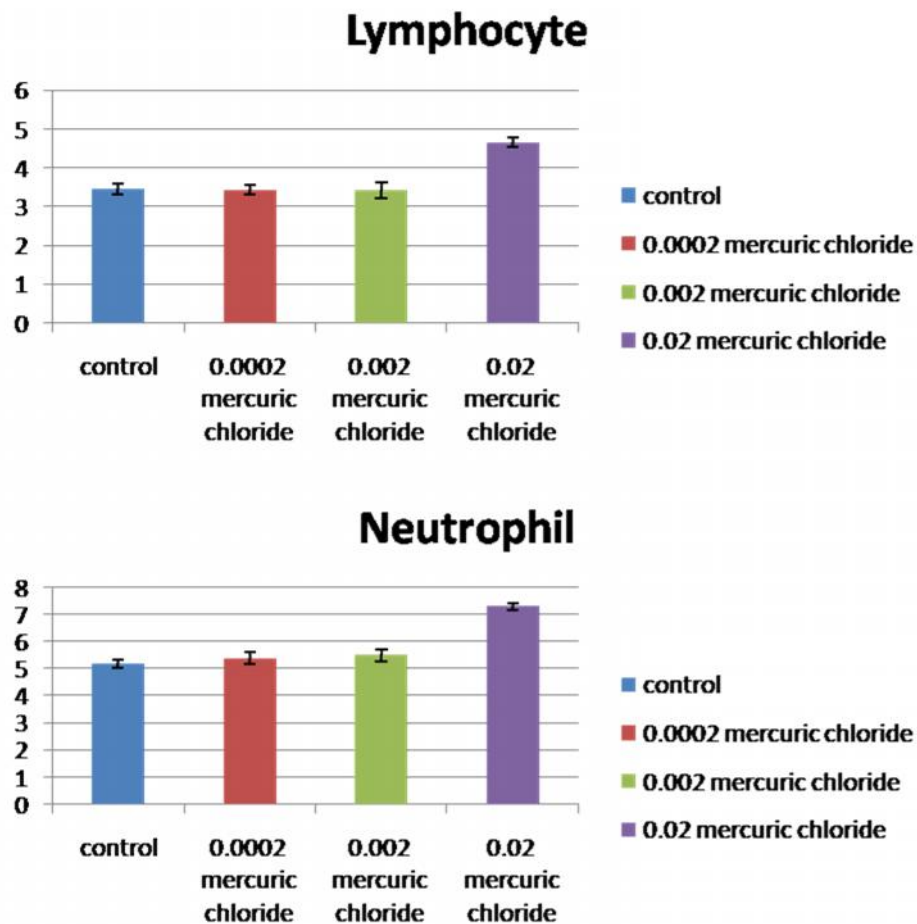
Fig.6: Differences in WBCs count ( \times 10^3 cells/mm 3 ) in all experimental groups.
