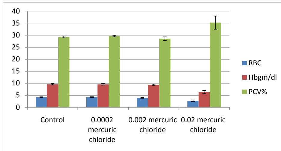
Fig.2. Changes in RBCs count (x10 6 cells/mm 3 ), Hb concentration (gm/dl) and PCV (%) in all experimental groups.
