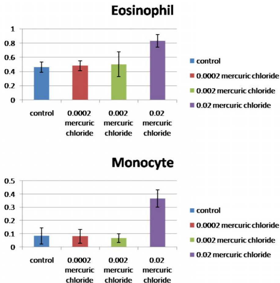
Fig.8: Changes in Eosinophil and Monocyte (x10 3 cells/mm 3 ) in all experimental groups.
