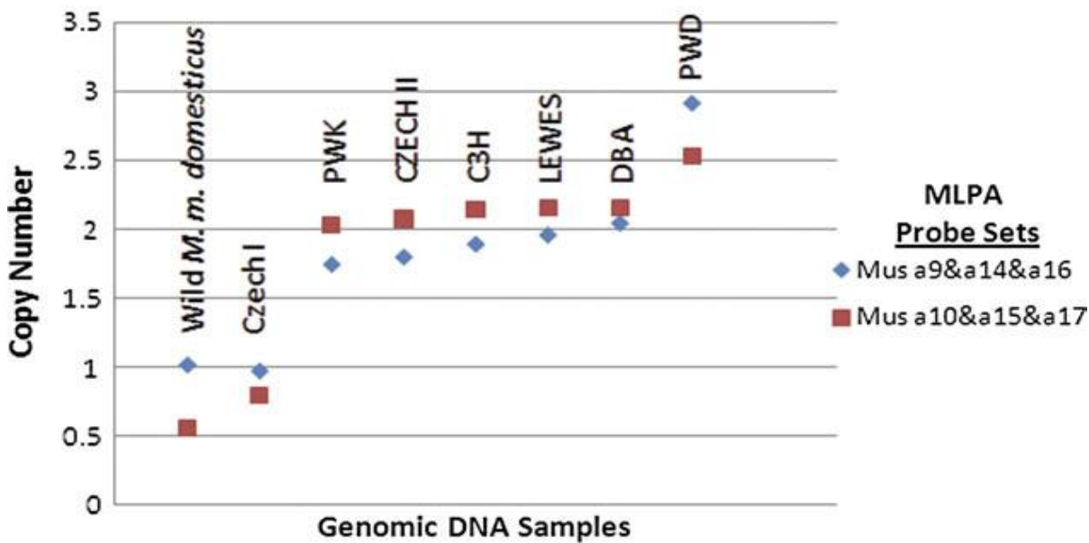
Figure 4. CNV of a9p/a14p/a16p , and a10/a15/a17 . Multiplex ligation probe assay (MLPA) was used to quantitate copy number. DNA probes specific for each group of paralogs were annealed to genomic DNA and subjected to ligation. Polymerase chain reaction of the ligated products was conducted with primers specific for the tails on the probe oligomers. The graph shows the copy number for each probe set indexed to values for known single-copy genes.
