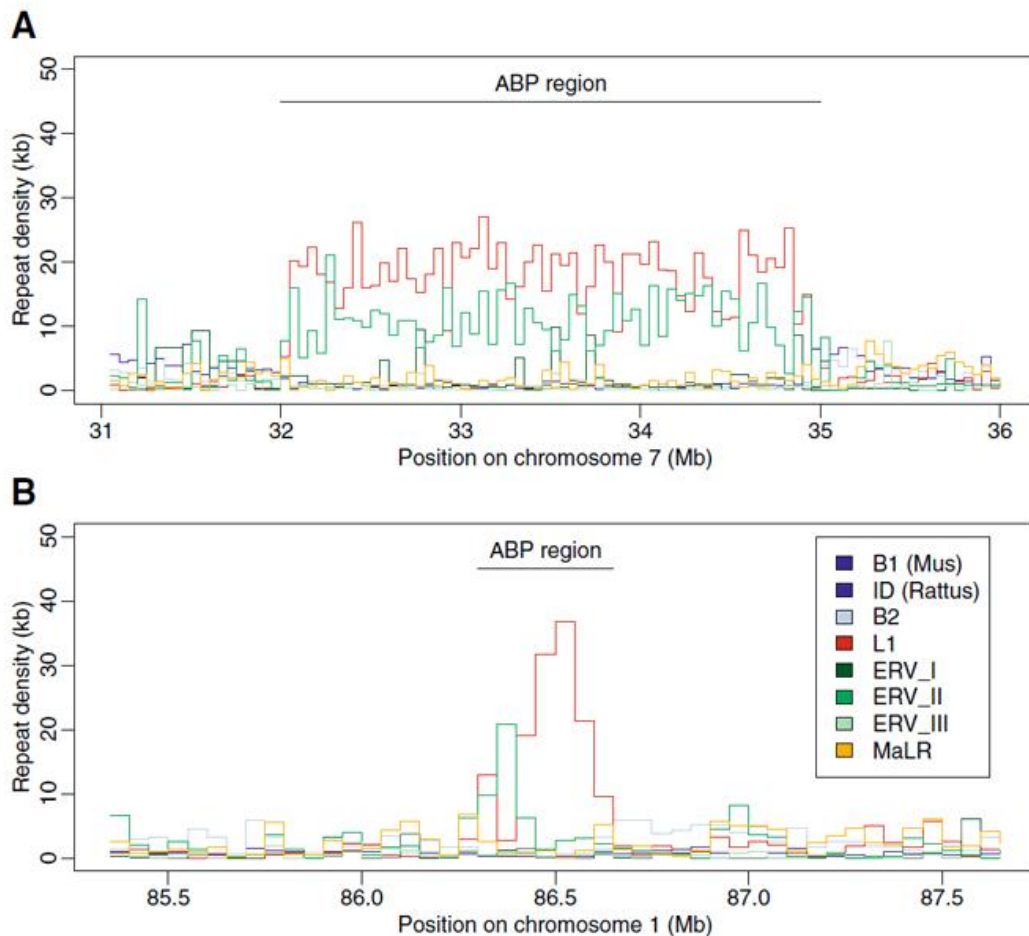
Figure 6. Densities of repeat families on chromosome 7 in mouse (A) and chromosome 1 in rat (B) genomes within 50 kb windows plotted along the physical position of the chromosome in the Abp gene family regions and their one Mb flanking regions. Densities are based on the RepeatMasker output provided at the UCSC Genome Browser website for mouse (NCBI M37/mm9) and rat (Baylor 3.4/rn4) genomes.
