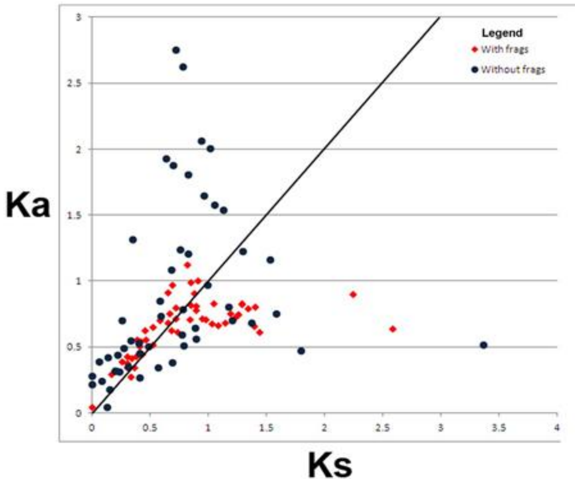
Figure 4. Ka plotted vs. Ks for selected mouse Esp sequences. The line demarcates a slope of 1.0. Each sequence is plotted twice. The red diamonds mark the Esp sequences including inner fragment sequences and the blue dots show the same Esp sequences with the inner fragment sequences removed.
