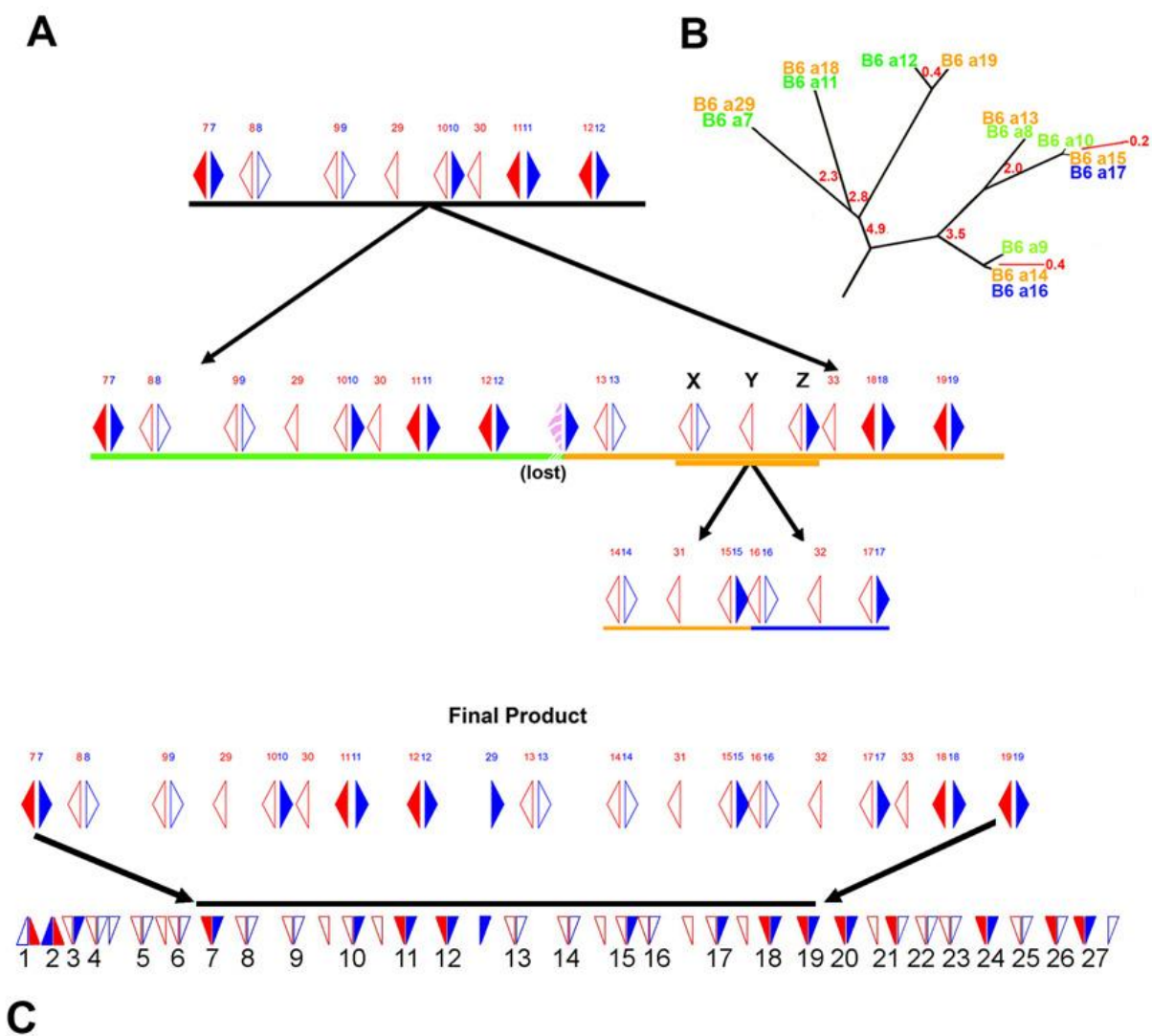
Figure 7. A model for recent Abp gene duplication events. (A) Partial map of Abp genes with arrows
