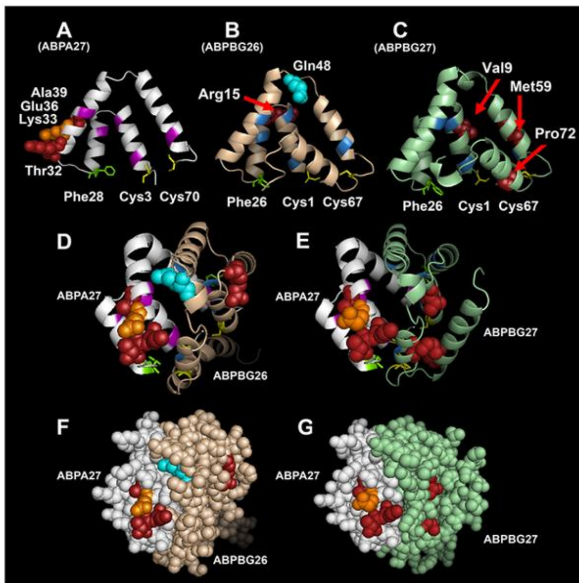
Figure 11. Positive selection at sites on molecular models of mouse salivary ABPA27 and ABPBG26 and the dimer they form. Panels A–E are cartoon-format models with spiral ribbons representing alpha helices and thinner connecting lines representing loops. Gene trees were used for the CODEML analyses of the coding regions of bg26 and a27, the species tree for bg27. Panels F and G are illustration of the dimers composed of the two subunits with amino acid residues as filled spheres. Panels A–C show inside views of the three ABP subunits: ABPA27 (white), ABPBG26 (tan) and ABPBG27 (light green), respectively. The conserved residues that line the ligand-binding pocket are represented in purple for the ABPA27
