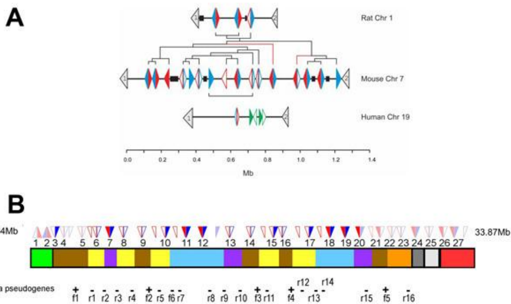
Figure 1. The Abp gene family linkage groups from [68] and from [25]. (A) A graphical representation of the relative position and transcriptional orientation of the Abpa - and Abpbg -like genes and pseudogenes located on Rattus norvegicus chromosome 1, Mus musculus chromosome 7, and Homo sapiens chromosome 19. The 5'–3' orientations of the genes are shown by the direction of the arrowheads. Scn1b and Uble1b genes, which lie in orthologous genomic regions in all three species, are numbered 1 and 2, respectively. Abpa -like genes are shown in blue, Abpbg -like genes in red, and primate SCGB4A1-4(P) genes in green. Filled arrowheads represent predicted functional genes; open arrowheads denote predicted pseudogenes. The sequence of duplication events among rodent genes inferred from phylogenetic trees is implied from the dendrogram, shown in black. Blue and red lines in this dendrogram represent branches that are not supported by the phylogenetic trees shown in [68]. The scale bar shows approximate genomic distance in megabases. Gaps (>5 kb) in the genomic assembly of each species are shown as black boxes. (B) A graphical representation of the relative position and transcriptional orientation of the Abpa and Abpbg genes and pseudogenes located on Mus musculus chromosome 7. Predicted genes and pseudogenes are indicated as filled and unfilled triangles, respectively. Abpa paralogues are shown in blue and Abpbg paralogues are shown in red. The original paralogues of [68] are faded, while the new paralogues described by [25] are in bright colors. Ribosomal protein L23a pseudogenes on the forward and reverse
