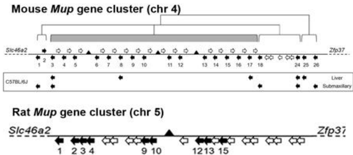
Figure 9. The mouse Mup gene cluster. Black arrows indicate direction of coding genes, numbered beneath, in the mouse genome. White arrows indicate direction of pseudogenes. Gaps in the genome are indicated by black triangles. The genes are arranged in two classes based on phylogeny, Class A in open brackets and Class B shaded grey. Genes expressed in male C57BL/6J liver and submaxillary glands indicated by black arrows, by RNA expression analysis.
