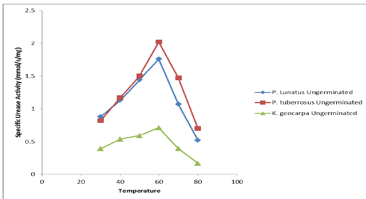
Figure 2.2a: Effect of temperature on urease activity (ungerminated beans)
