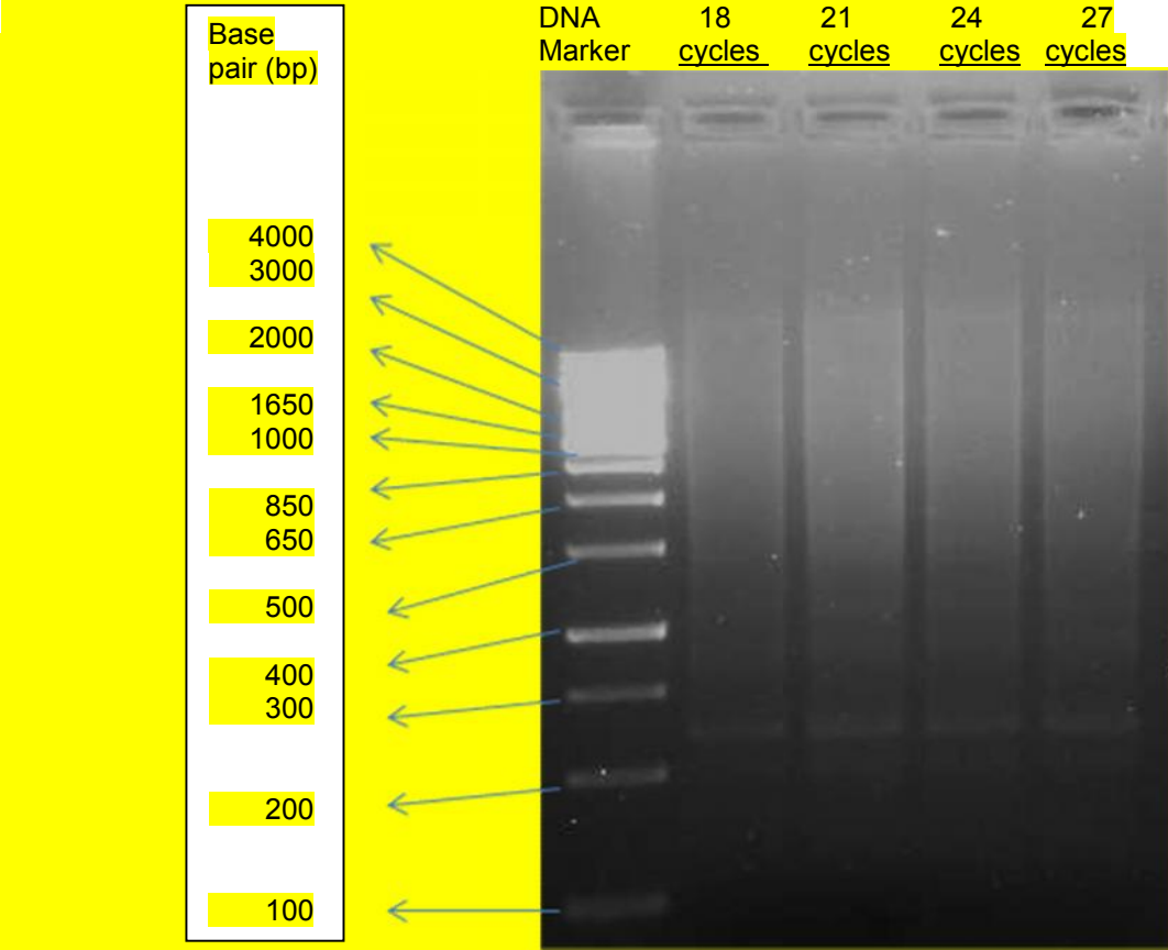
251 Figure 2 : LD PCR cycles yielding smear ranging in size from 0.1 to 4 Kb.
