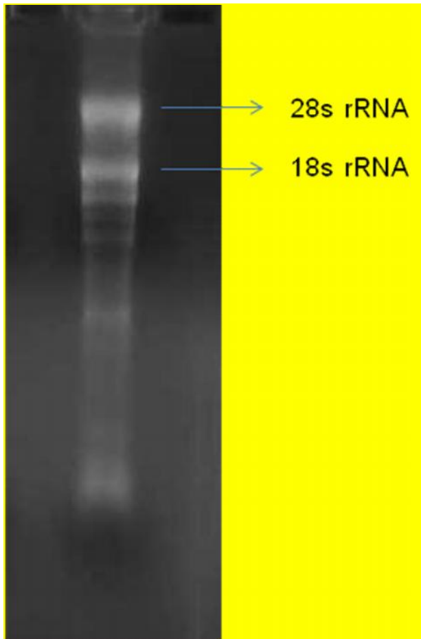
Figure 1: 1.5% agarose-formaldehyde gel showing RNA isolated from fresh young leaves of P. amarus .
