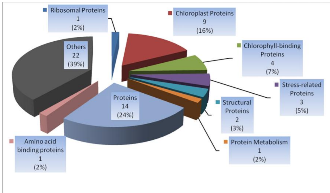
Figure 3: Functional categorization of 57 sequences into nine classes according to BLASTX analysis.
