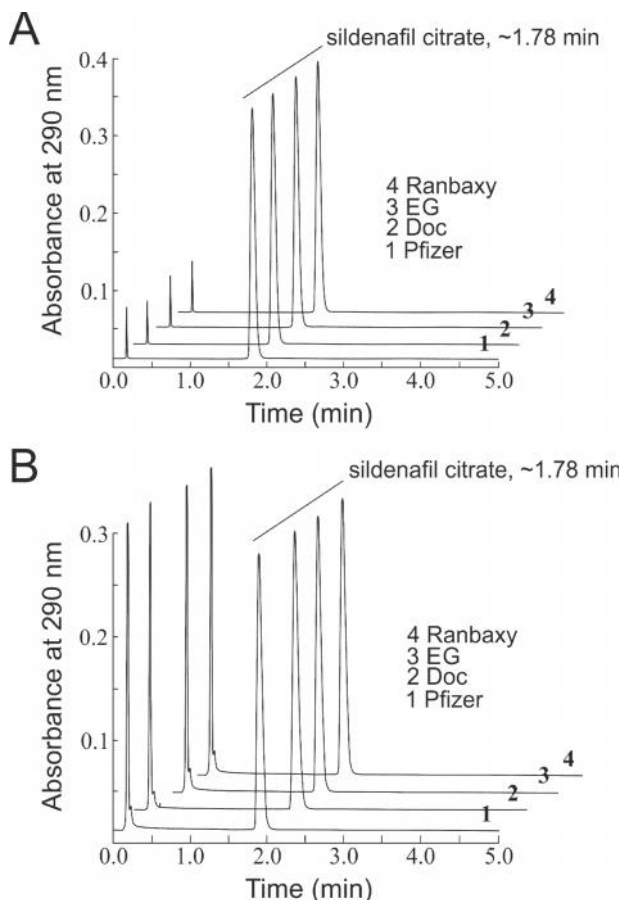
135 Fig. 2: Elution profiles of Italian market formulation of Viagra samples (50 mg tablets from 136 Pfizer, DOC generic, EG SpA, Ranbaxy Italia SpA) after chemical treatment under 137 acid (A) or basic (B) conditions.
