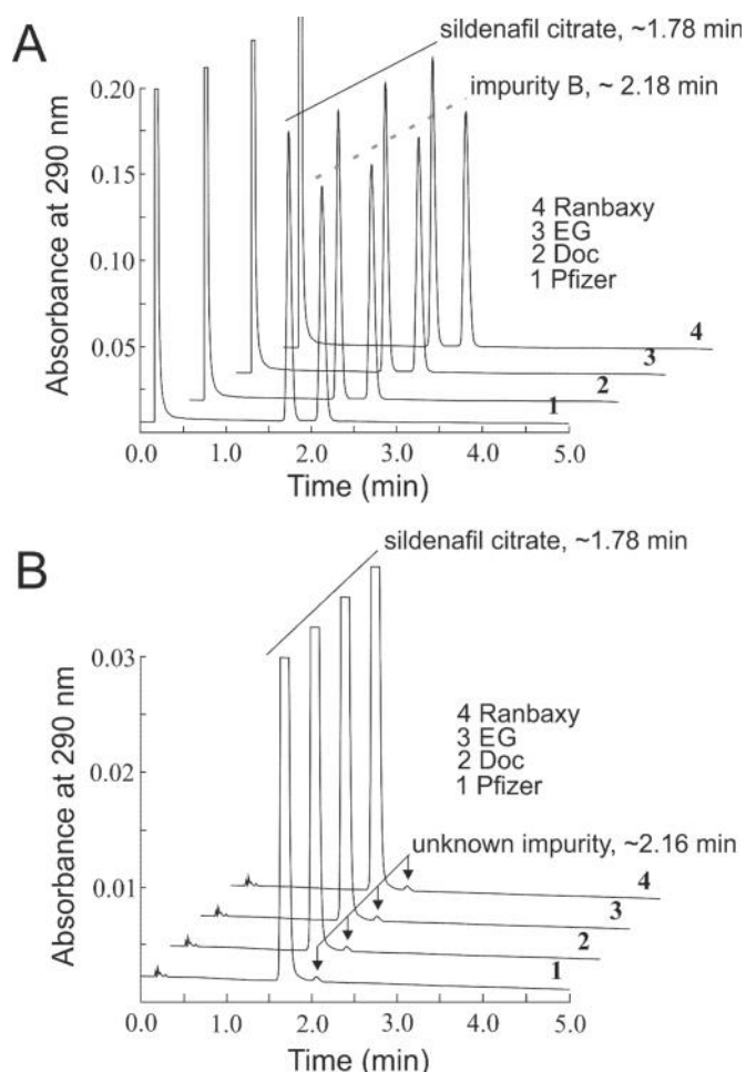
Fig. 3: Elution profiles of Italian market formulation of Viagra samples (50 mg tablets from Pfizer, DOC generic, EG SpA, Ranbaxy Italia SpA) after chemical treatment with hydrogen peroxide (A) or heating (B) conditions.
