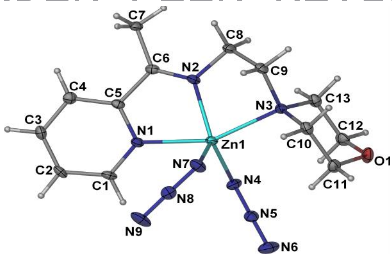
Fig. 1. Crystal structure for [Zn(N 3 ) 2 (C 13 H 19 N 3 O)]
