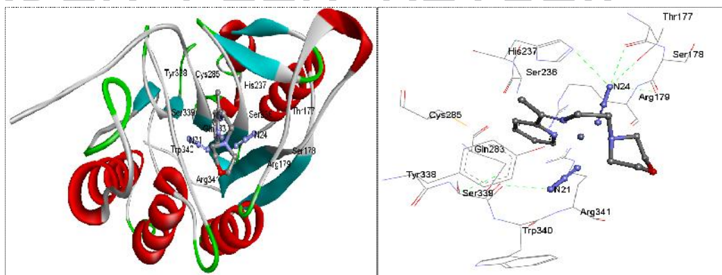
Fig. 2. Representations of the molecular model of the complex formed between \text{Zn(LMA)(N}_3)_2 and caspase 3 zymogen. And 3D representation of the ligand-enzyme binding interactions. \text{Zn(LMA)(N}_3)_2 Compound is represented as a dark grey sticks and hydrogen bonds as green dashed lines
