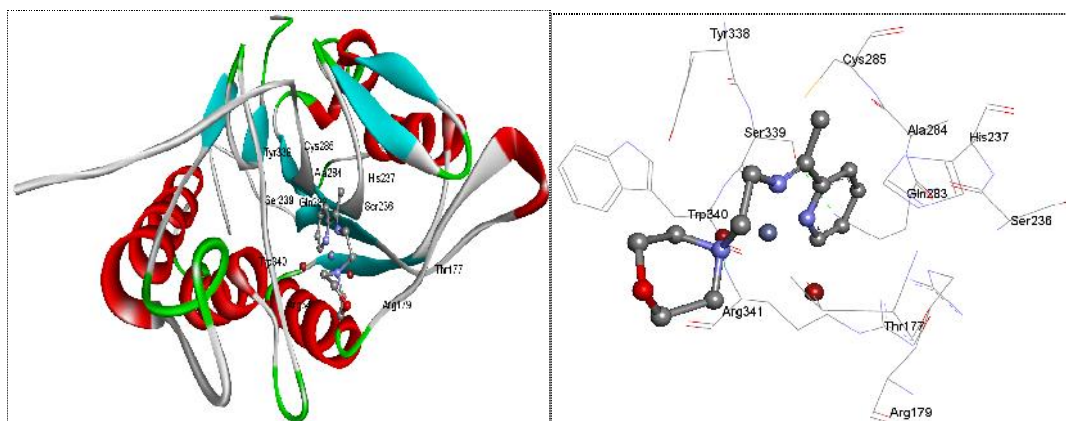
Fig. 3. Representations of the molecular model of the complex formed between \text{Zn(LMA)Br}_2 and caspase 3 zymogen. And 3D representation of the ligand-enzyme binding interactions. \text{Zn(LMA)Br}_2 Compound is represented as a dark grey sticks and hydrogen bonds as green dashed lines
