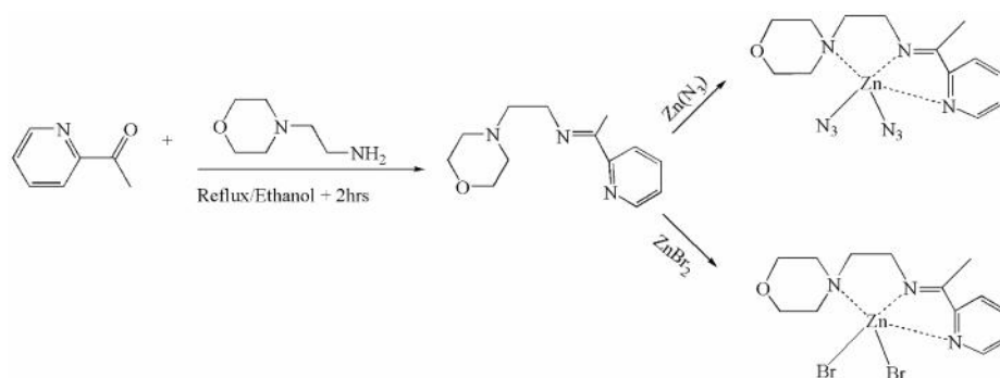
Scheme 1. Molecular structures of the zinc(II) ion complexes
