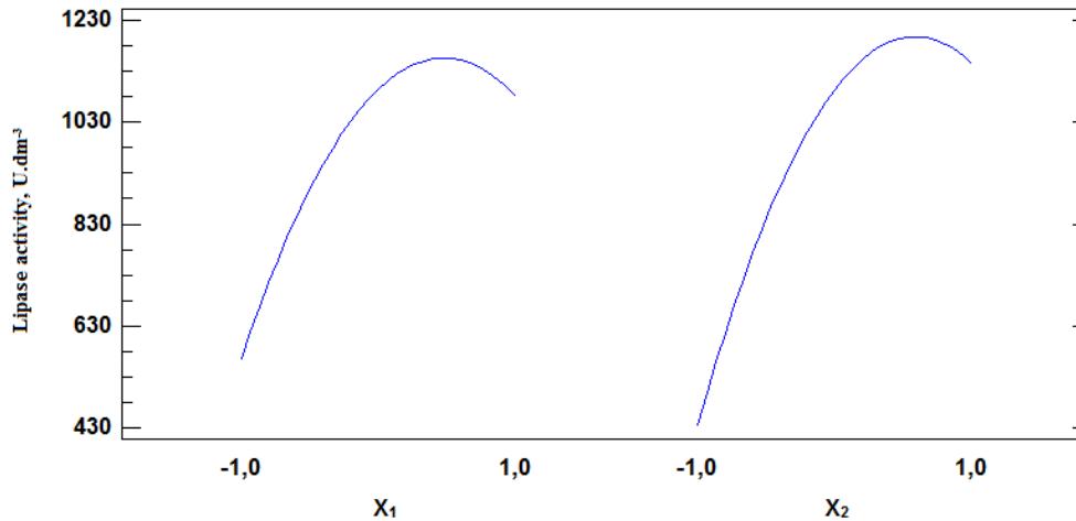
Fig. 2. Main effects plot
