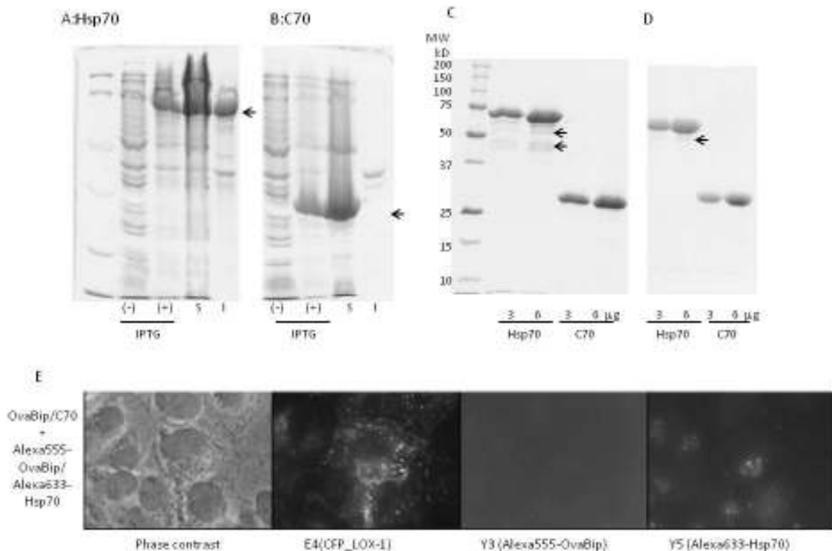
207 Fig.2. Expression and stability of recombinant Hsp70 and C70. Recombinant Hsp70 208 and C70 were purified as described in material and methods. E. coli bacterial cell lysates 209 and purified proteins were examined by SDS-PAGE and proteins were visualized by 210 Coomassie staining. (A) Hsp70, (B) C70. (-): bacterial culture without IPTG, (+) with IPTG for 211 4 h; S: soluble fraction, I: insoluble fraction. Arrows indicate the expected molecular mass of 212 Hsp70 or C70. (C) Hsp70 and C70 eluted from Ni-NTA Agarose column. Each lane 213 contained 3 µg or 6 µg total proteins. Arrows indicate contaminating protein. (D) Stability of 214 Hsp70 and C70. Purified proteins were stored at 4°C for 3 months and 3 µg or 6 µg total 215 proteins were run in each lane. Arrow indicates the degraded Hsp70. (E) HEK293 cells 216 stably expressing CFP_LOX-1 incubated with OvaBip/C70 followed by incubation with 217 Alexa555-OvaBip/ Alexa 633-Hsp70. 218 219
