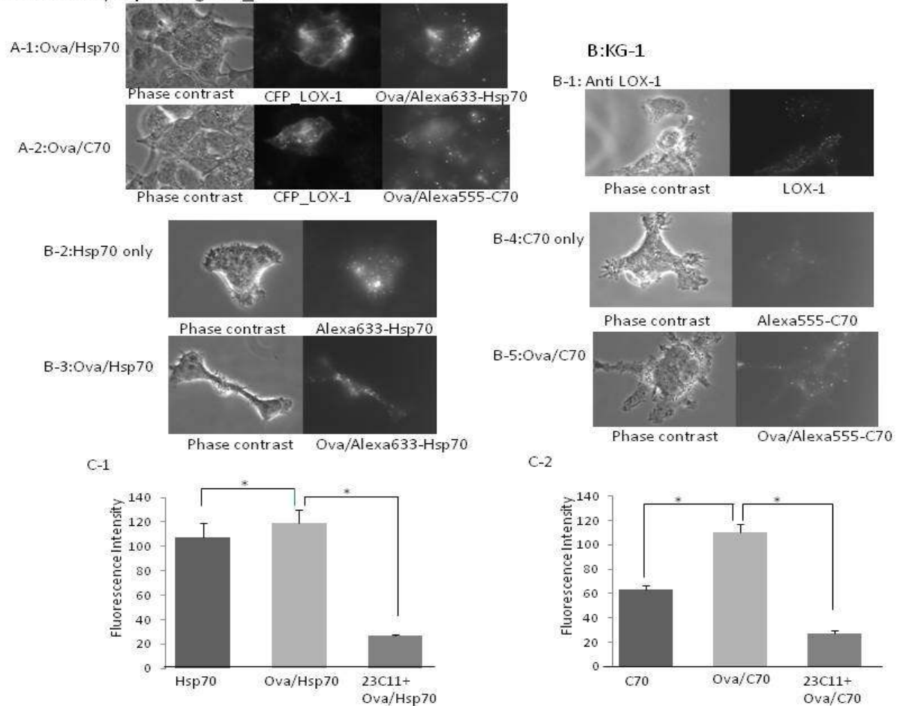
278 Fig. 4. LOX-1 is the receptor for uptake of Ova/Hsp70 and Ova/C70. A: HEK293 cells stably 279 expressing CFP_LOX-1 incubated with Ova/Alexa633-Hsp70 (A-1) or Ova/Alexa555-C70 (A- 280 2), and then examined by fluorescence microscopy. B: KG-1 cells were differentiated into 281 DCs, incubated with proteins or peptide/protein complexes, and then examined by 282 fluorescence microscopy. (B-1) DCs stained with anti-LOX-1 antibody. (B-2) DCs incubated 283 with Alexa633-Hsp70. (B-3) DCs incubated with Ova/Alexa633-Hsp70. (B-4) DCs incubated 284 with Alexa555- C70. (B-5) DCs incubated with Ova/Alexa555-C70. (C) DCs incubated with 285 LOX-1-neutralizing antibody (23C11) followed by incubation with Ova/Alexa633-Hsp70 or 286 Ova/Alexa555-C70. Images of over 100 DCs from 3 independent experiments were 287 acquired. Fluorescence intensity was quantitatively evaluated using region-measurement 288 analysis (MetaMorph) as described in Material and Methods. Data are expressed as the 289 fluorescence intensity after subtracting the background emission level \pm SD, *P < 0.05 290 291 292
