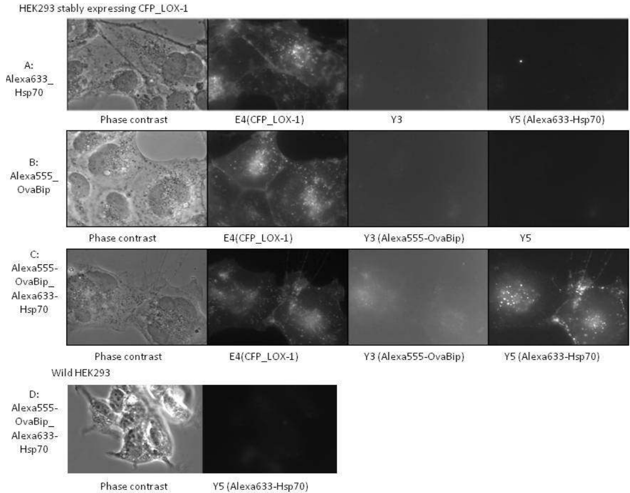
Fig. 1. LOX-1 is the receptor for uptake of Hsp70 and OvaBip complex. HEK293 cells stably expressing CFP_LOX-1 incubated with Alexa633-Hsp70, Alexa555-OvaBip, or Alexa555-OvaBip/Alexa633-Hsp70, and then examined by fluorescence microscopy. (A) Cells incubated with Alexa633-Hsp70. (B) Cells incubated with Alexa555-OvaBip. (C) Cells incubated with Alexa555-OvaBip/Alexa633-Hsp70. (D) Wild HEK293 cells incubated with Alexa555-OvaBip/Alexa633-Hsp70.
