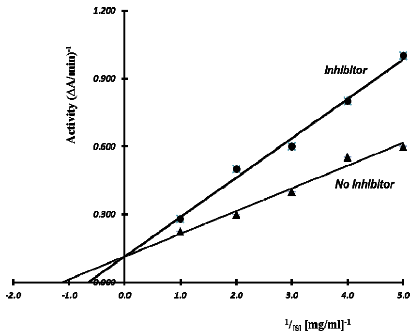
Figure 4. Lineweaver Burke kinetic plot of the effect of volatile oil of Thaumatooccus danielli (Benn.) Benth. (as inhibitor) against the caseinolytic activity of the extracellular protease of Shigella dysenteriae
