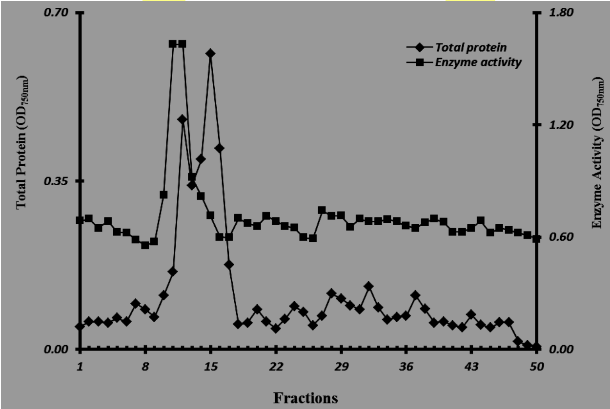
Figure 1. Sephadex G-75 elution chromatogram of the extracellular protease of Shigella dysenteriae (Fractions 10 – 13 were pooled and tagged as “partially purified enzyme”)
