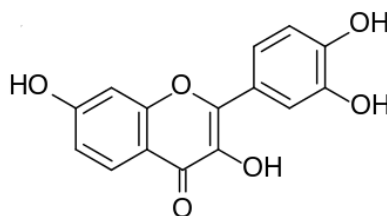
Fig. 1. The molecular structure of fisetin
