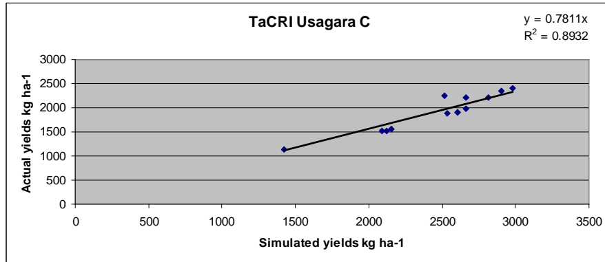
Figure 3a: Simulated and actual parchment yields, TaCRI Usagara C
