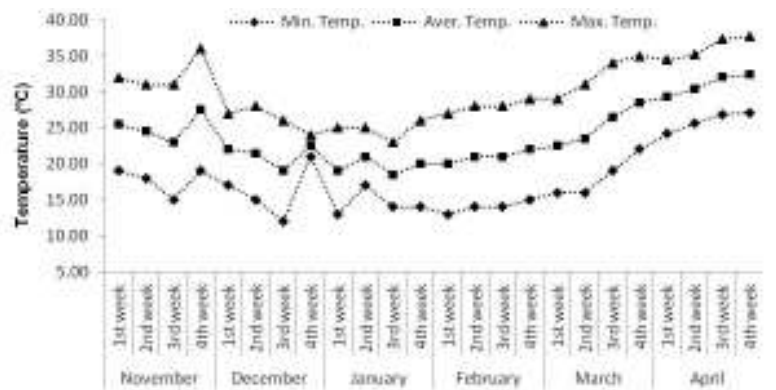
Weekly maximum, minimum and average temperature in Dhaka region
