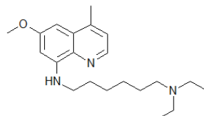
Figure 6. Sitamaquine chemical structure
