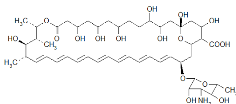
Figure 2. Amphotericin B chemical structure
