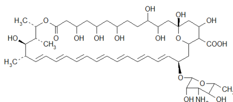
Figure 2. Amphotericin B chemical structure
