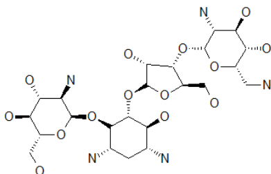
Figure 4. Paromomycin chemical structure
