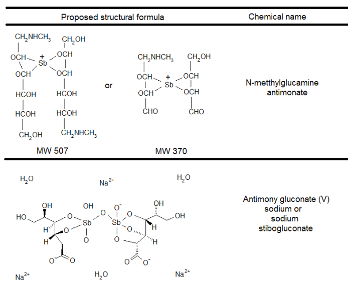
Figure 1. Proposed chemical structure of antimonials [13, 14]
