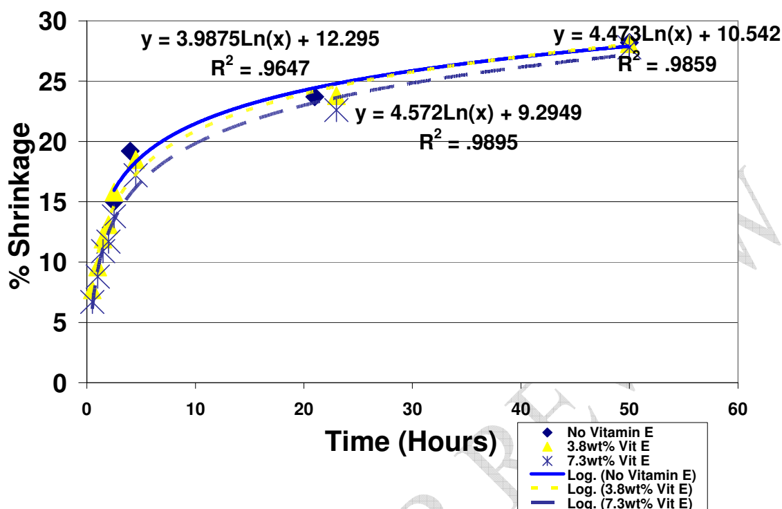
Figure 14. Lipid and Acrolein Polymerization Shrinkage with Vitamin E
