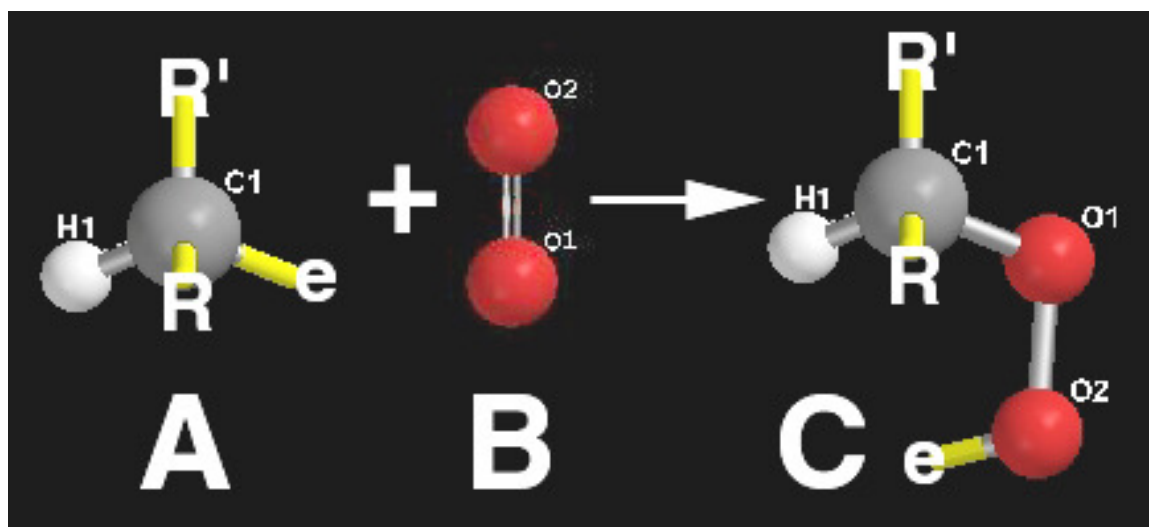
Figure 2. Lipid peroxidation of the carbon tetrahedral from (A) a saturated lipid \text{-CH}_2\text{-} backbone group after hydrogen abstraction to form a carbon-centered free radical and then subsequent combining with (B) molecular oxygen to form a (C) lipid peroxy free radical with large reactive electrophile swing rotation by two oxygen single bonds.
