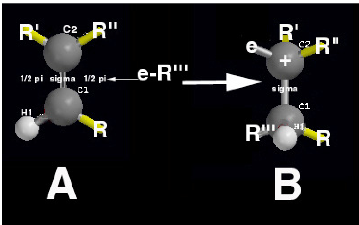
Figure 3. Reactive secondary sequence where (A) a lipid planar C=C alkene \pi bond is attacked by a free-radical electrophile with unpaired electron, e-R''' , to (B) form a carbon tetrahedral for an R''' \sigma single bond generally on the end carbon atom and produce a tertiary carbocation radical with a new unpaired electron on the opposite carbon atom.
