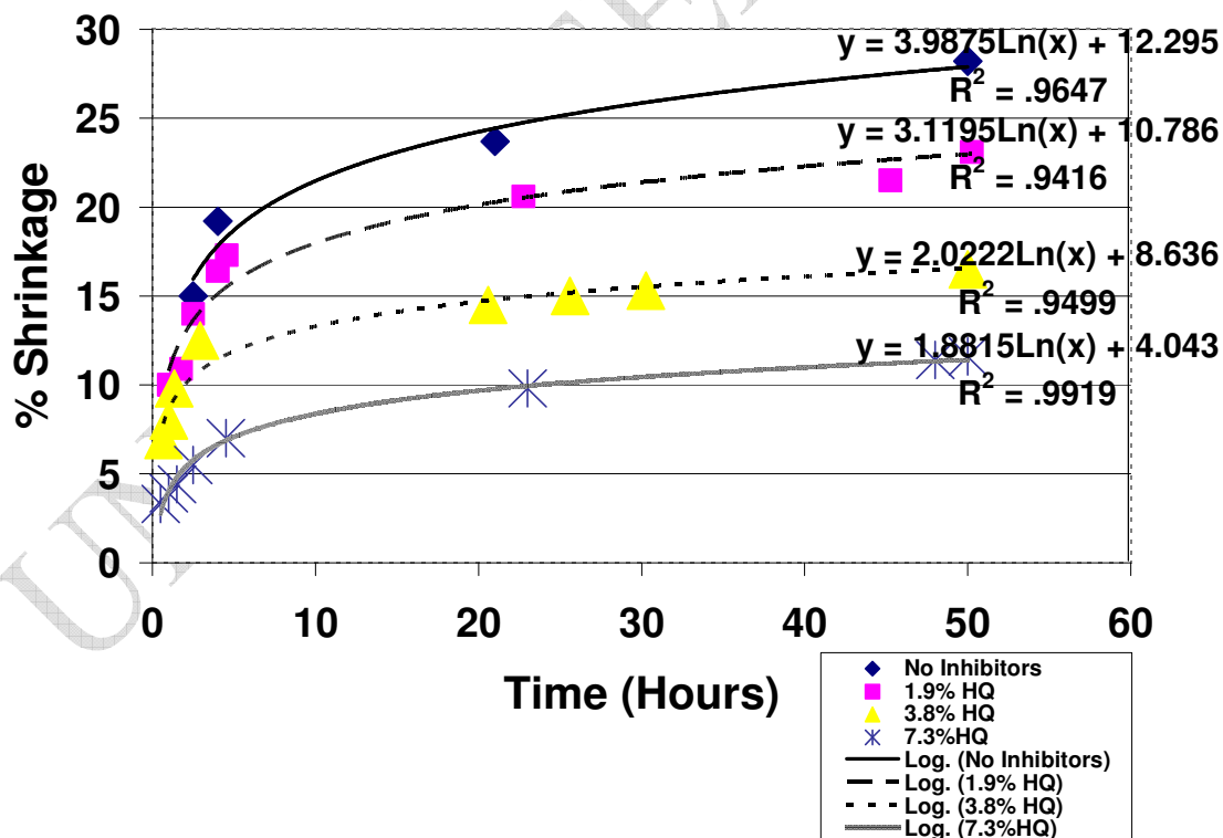
Figure 15. Lipid and Acrolein Polymerization Shrinkage with Hydroquinone (HQ)
