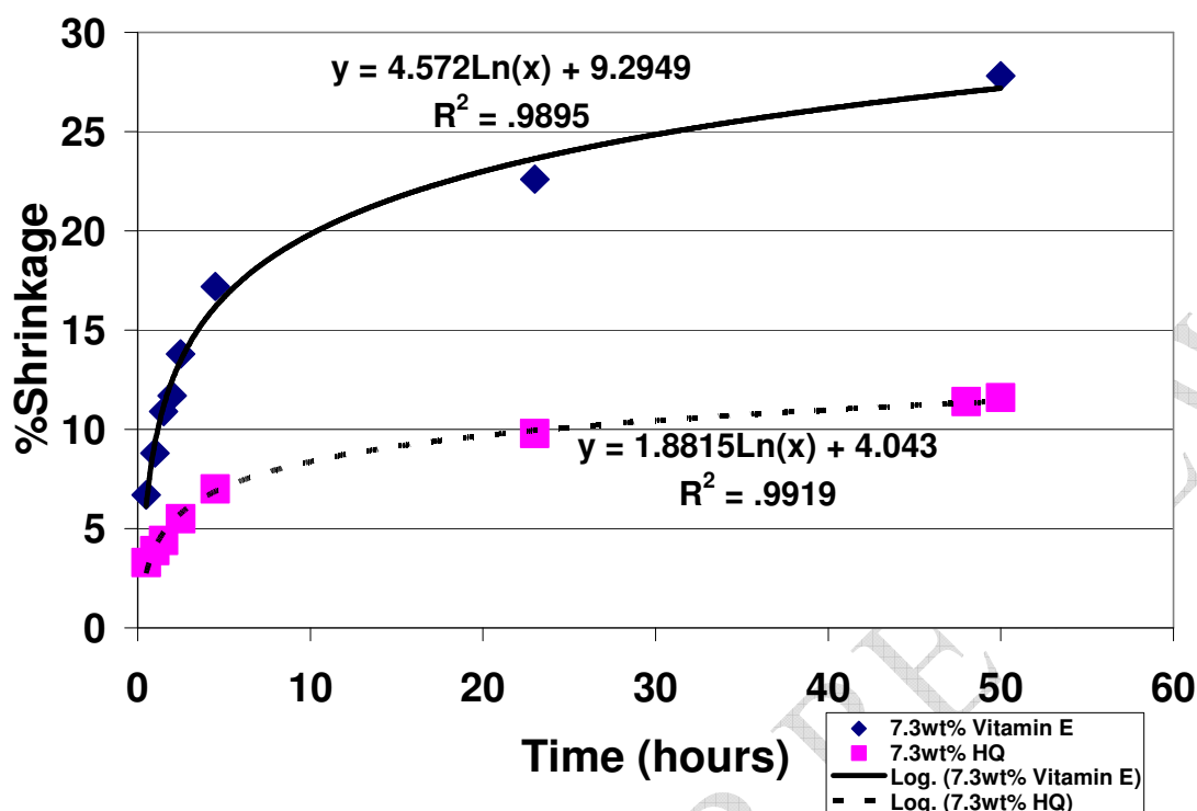
Figure 16. Lipid and Acrolein Polymerization Shrinkage Comparing 7.3% Hydroquinone (HQ) with 7.3% Vitamin E.
