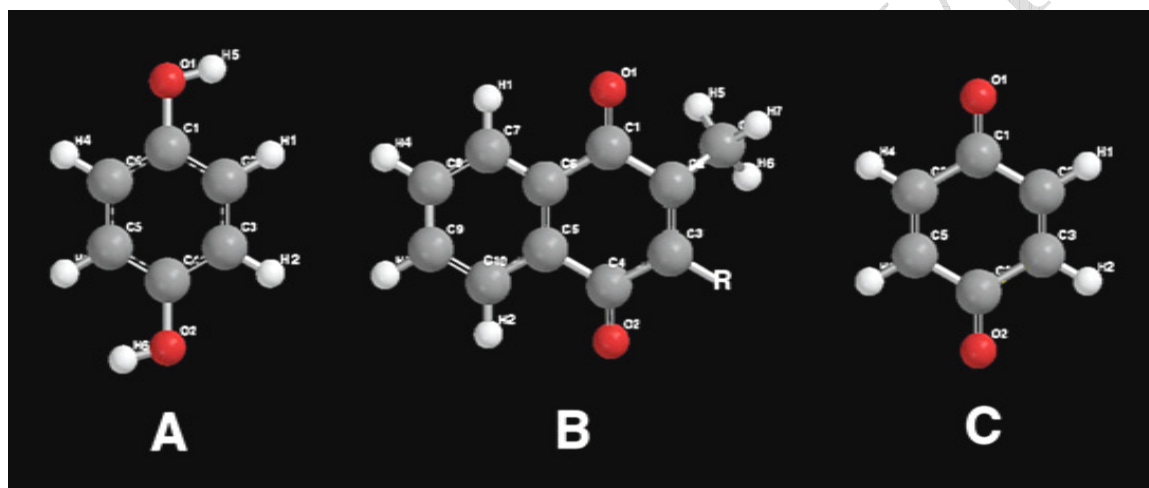
Figure 7. (A) Hydroquinone (B) Vitamin K shown in the reduced quinone form (C) Quinone
