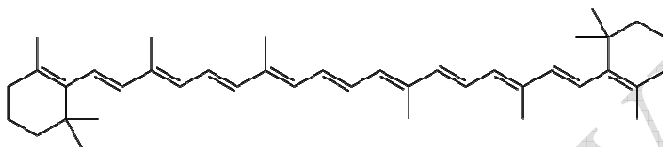
Figure 6. \beta,\beta -carotene conjugated C=C double-bond \pi system produces a deeply colored pigment and can be cleaved enzymatically into two molecules of vitamin A (McMurry, J. 2004).
