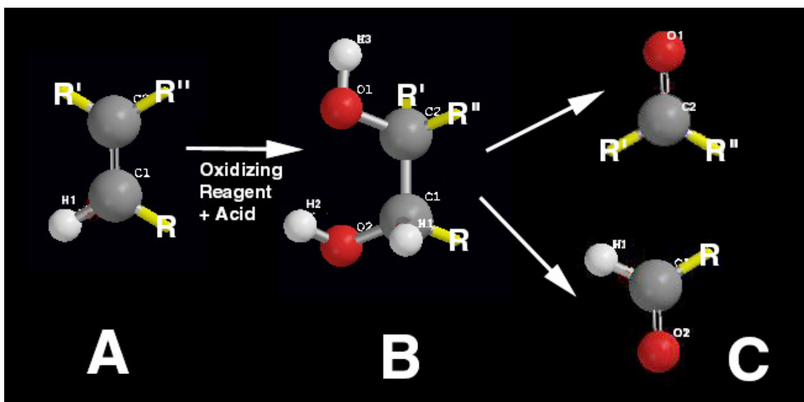
Figure 4. (A) Lipid Alkene (B) Glycol Oxidation intermediate (C) Oxidative Cleavage into Ketone top and Aldehyde bottom during highly concentrated free radical or combined acidic conditions.
