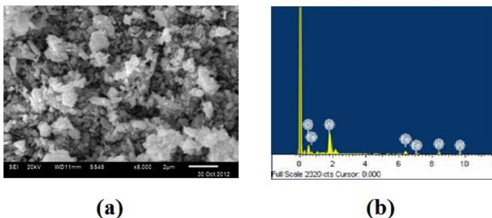
Fig. 6. a) SEM image of FeWO 4 powder and b) EDS of the FeWO 4 powder under SEM investigation.
