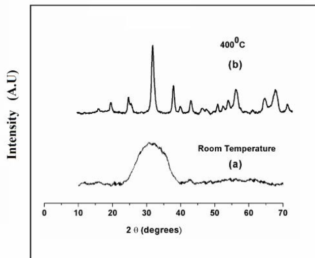
Fig. 2. XRD patterns of stiochiometric mixture of \text{ZnCl}_2 + \text{Na}_2\text{WO}_4 ground for 2hrs a) room temperature, b) heat treated at 400^\circ\text{C} for 4hrs
