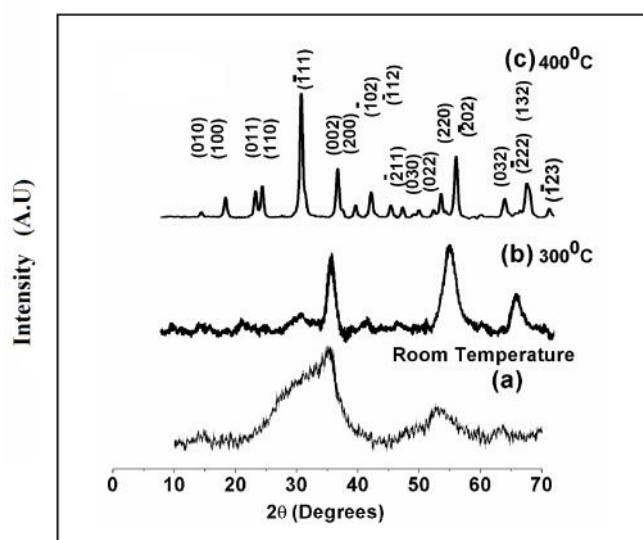
Fig. 1. XRD patterns of stoichiometric mixture of NiCl_2 + Na_2WO_4 ground for 2hrs a) room temperature b) heat treated at 300^\circ C for 4hrs c) heat treated at 400^\circ C for 4hrs and washed free of chloride.
