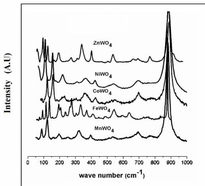
Fig. 5. Raman spectra of MnWO_4 , CoWO_4 , NiWO_4 and ZnWO_4 heat treated at 400^\circ\text{C} and FeWO_4 heat treated at 600^\circ\text{C} .
