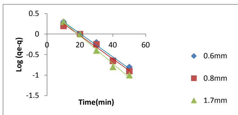
Fig.14. Relationship between different particle size and time of adsorption.
