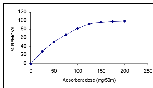
Fig.5.Effect of Adsorbent dose on % removal of Cr(VI). Fig.6. Effect of adsorbent dose % removal of Ni (II)
