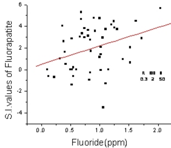
Fig. 4: Fluoride Vs S.I. values of Fluorapatite Mineral
