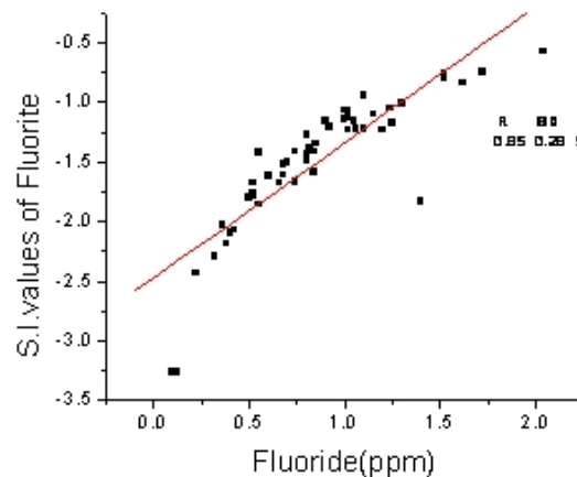
Fig. 5: Fluoride Vs S.I. values of Fluorite Mineral
