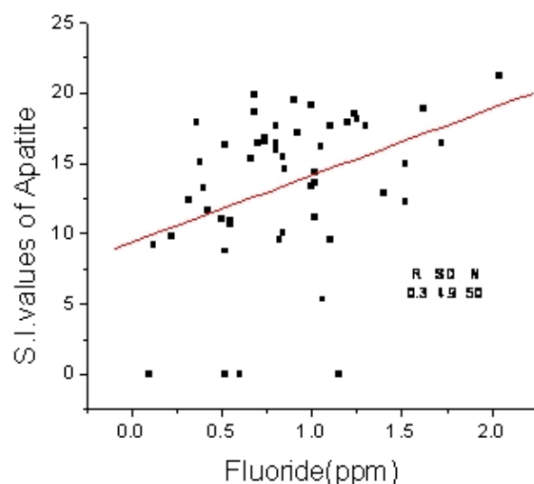
Fig. 3: Fluoride Vs S.I. values of Apatite Mineral
