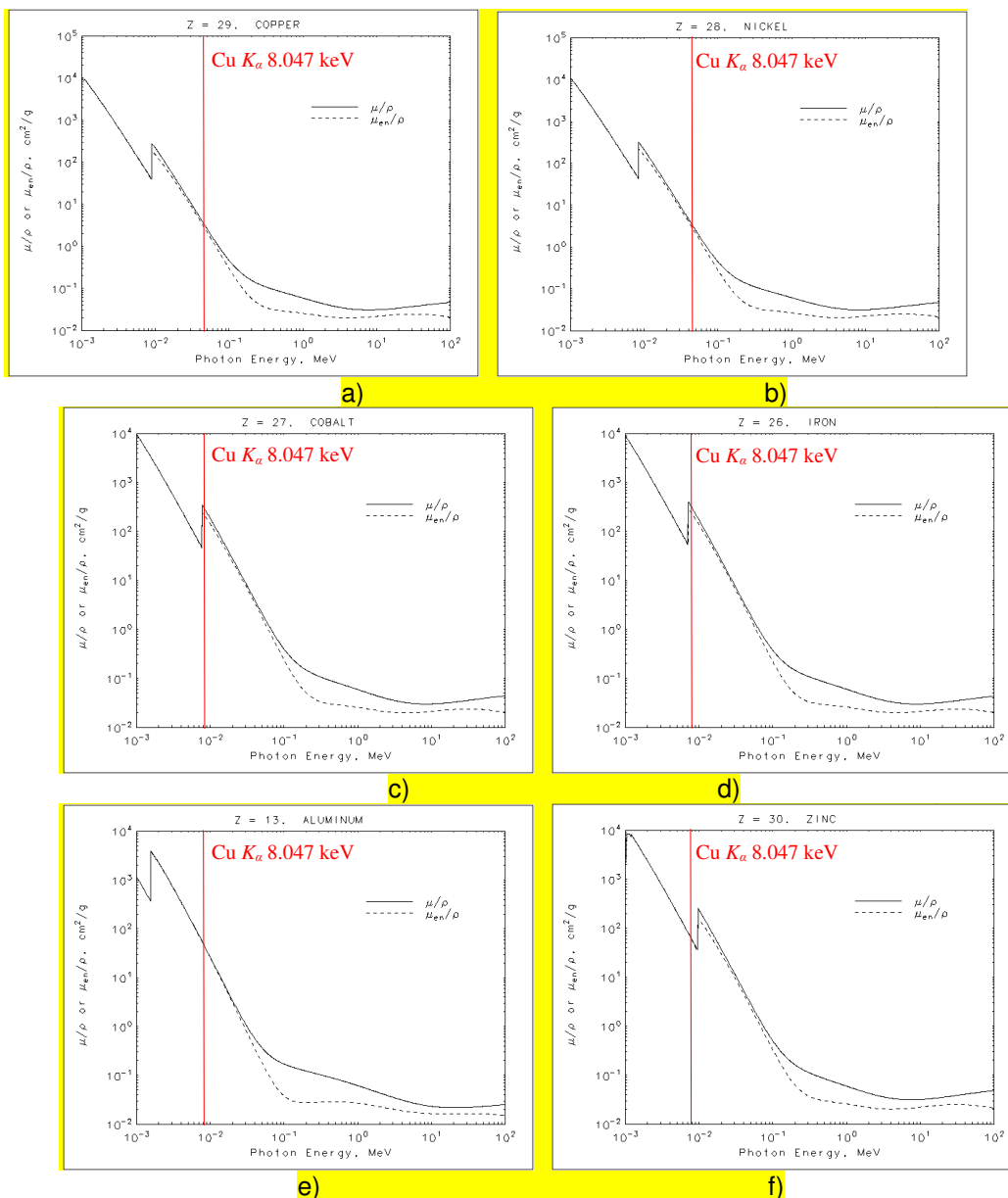
Fig. 5. Absorption curves of some elements of interest versus the most intensive luminescence of DPF through a copper K_{\alpha} -line centered at the 8.047-keV energy
