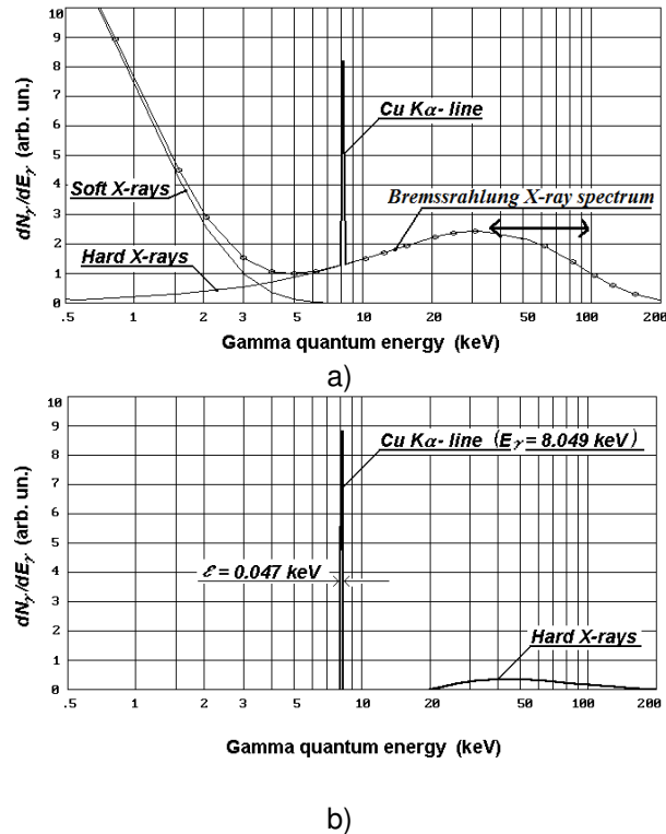
Fig. 3. The X-ray spectrum produced inside the chamber of the DPF device, and the DPF X-ray spectrum irradiated behind the 90-μm copper filter
