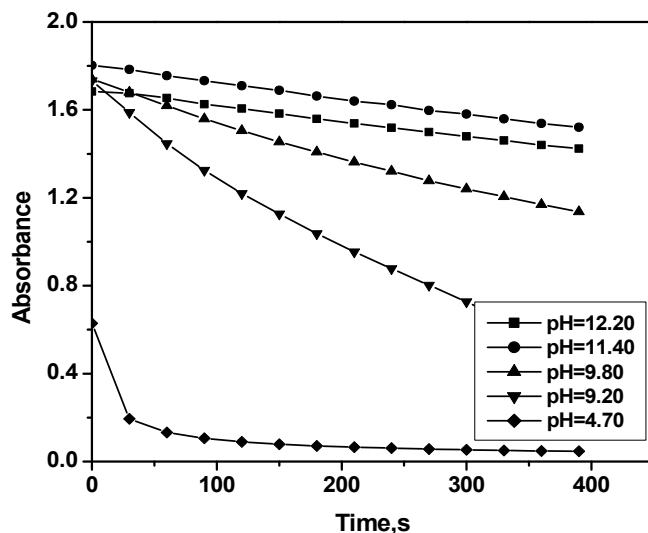
188 Fig. 3. Variation of absorbance versus time at different pH's. [GBP] = 0.01 mol dm -3 , 189 [NBS] = 0.1 mol dm -3 , and T = 20 °C
