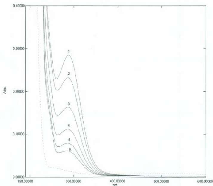
82 83 Fig. 1. Absorption spectra of the reaction mixture at different times. Peaks (1-6) were 84 recorded at 1, 2, 5, 10, 15, and 20 min. from the time of initiation of reaction 85 respectively. The dashed curve for aqueous solution of gabapentin alone. pH = 8.50, 86 T= 25°C , [GBP] = 0.001 mol dm -3 , [NBS] = 0.01 mol dm -3 87
