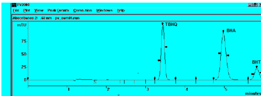
Figure 1. A typical chromatogram for standard antioxidants; BHT, BHA and TBHQ
