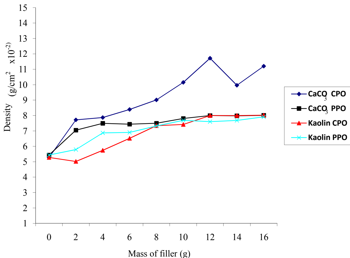
Fig. 2: Results of variations of CaCO 3 and kaolin filled CPO and PPO filler loadings with density.
