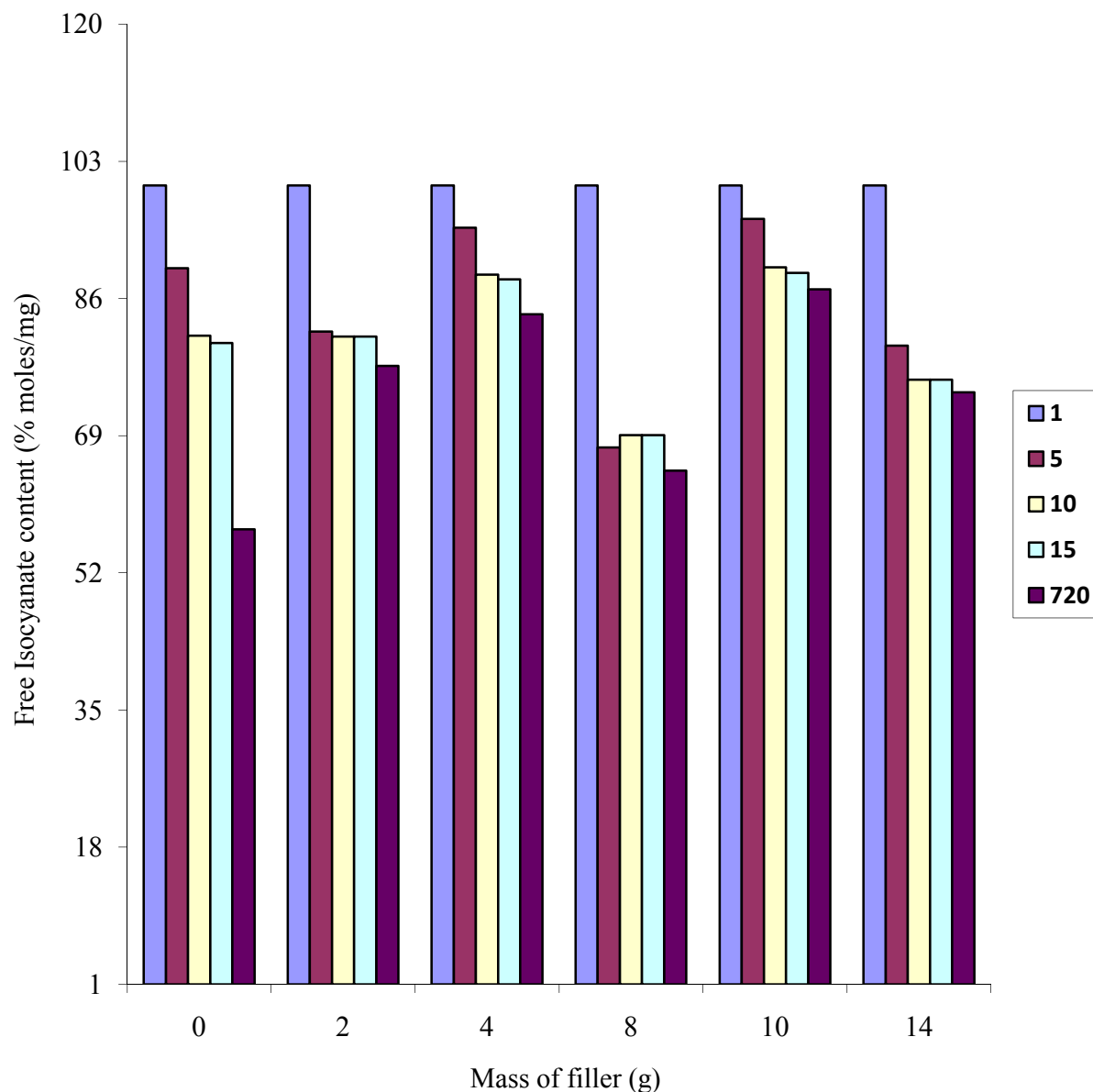
Fig. 6: Results of variations of Kaolin filled PPO with curing times.
