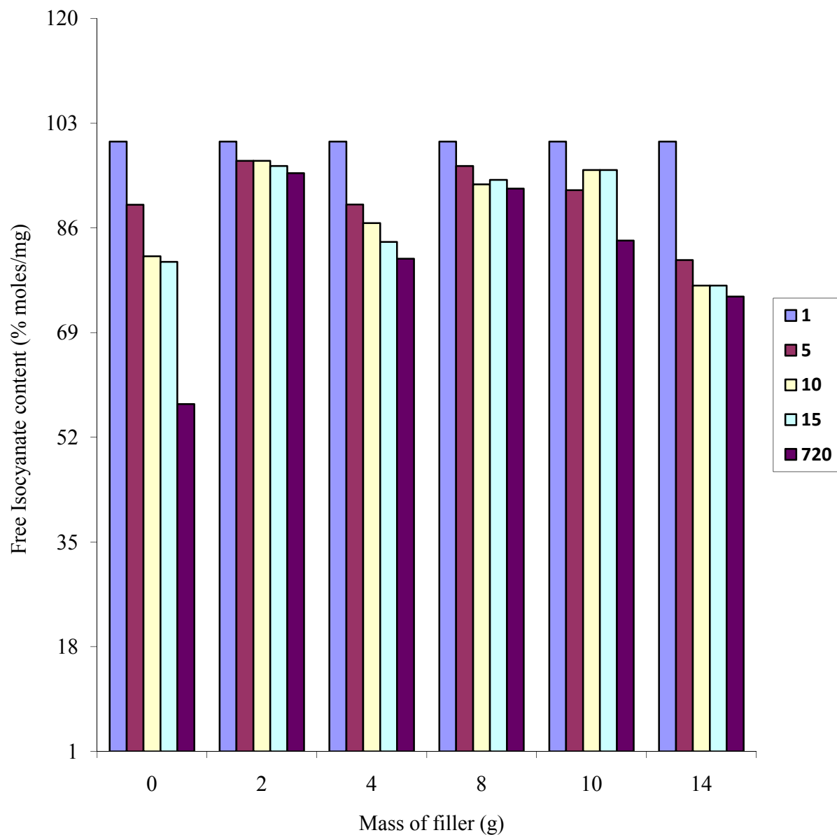
Fig. 5: Results of variations of \text{CaCO}_3 filled PPO with curing times.
