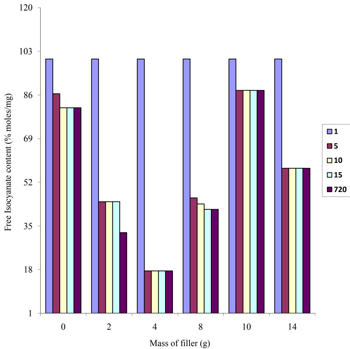
Fig. 4: Results of variations of Kaolin filled CPO with curing times.
