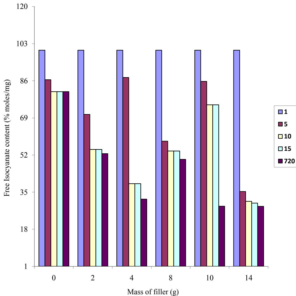
Fig. 3: Results of variations of \text{CaCO}_3 filled CPO with curing times.
