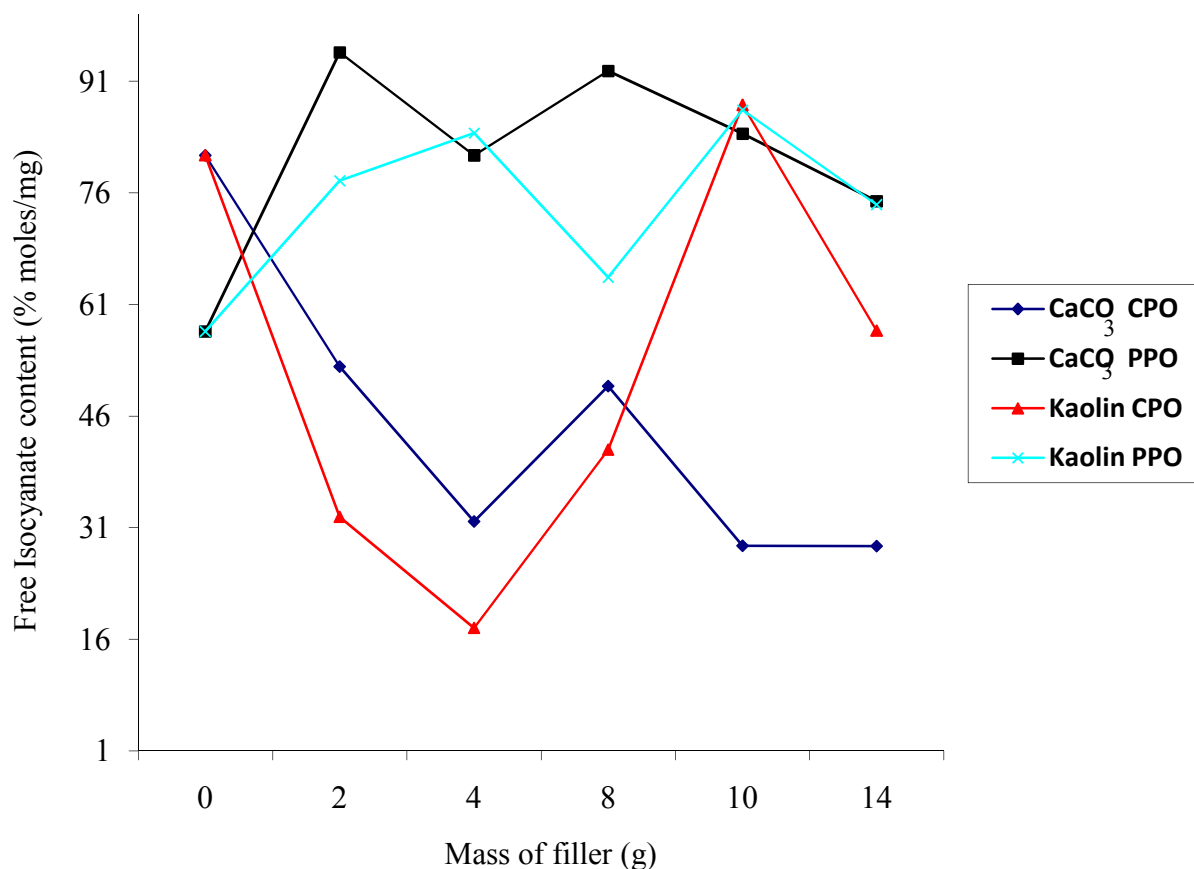
Fig. 7: Results of variations of % free Isocyanate content at aging times (720 mins).
