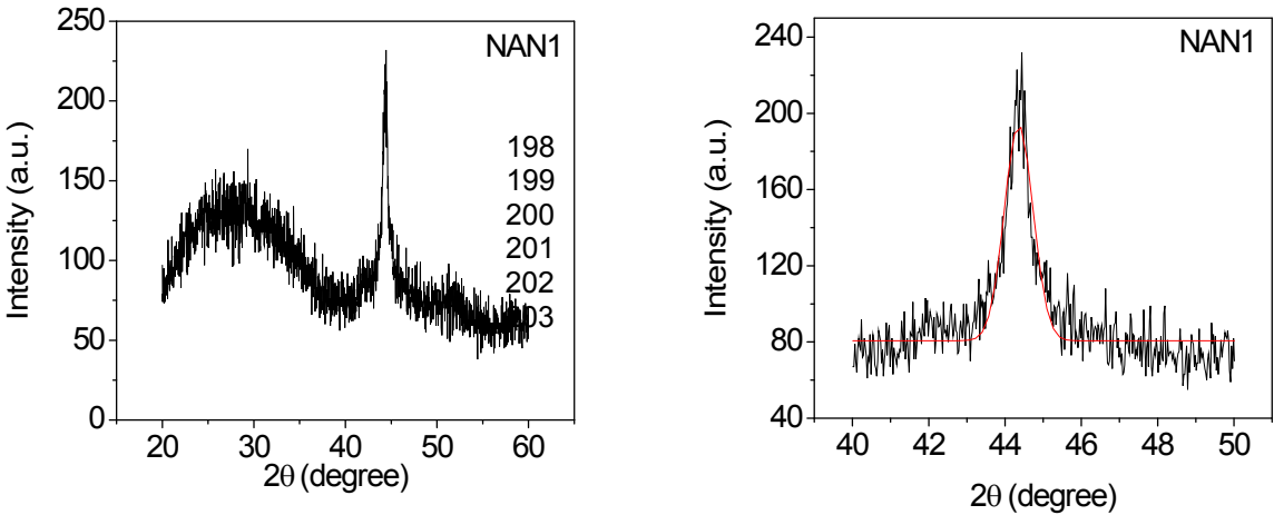
Fig.1. (a) XRD spectra for NAN1 film and (b) spectra around the peak position. The solid line is a Gaussian fit to the peak.
