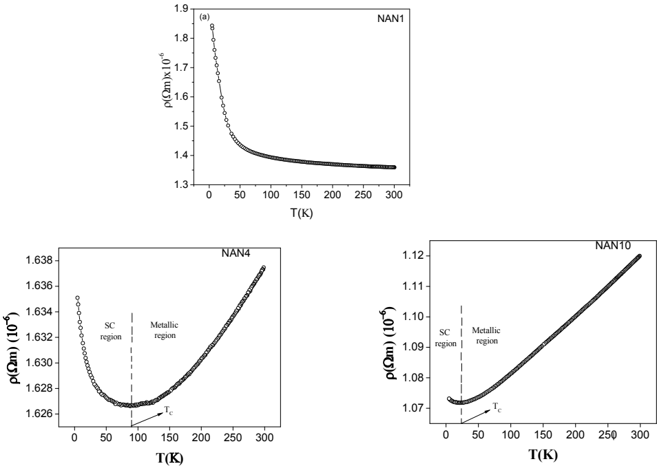
Fig.2: Temperature variation of resistivity of NAN1, NAN4 and NAN10
