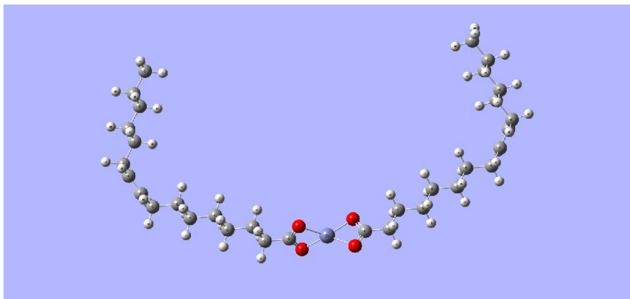
Figure 6: Optimized structure of zinc palmitoleate
