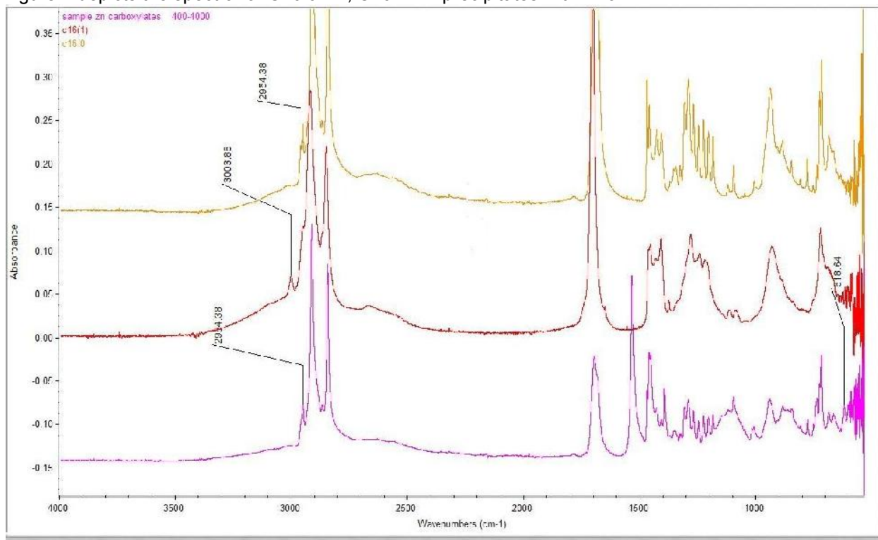
Figure 4: Spectra of C16:0 FA, C16:1 FA and Zinc Carboxylate precipitate
