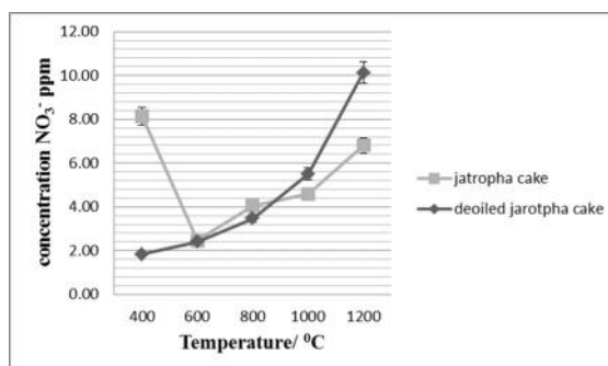
Figure 1: The effect of temperature on the amount of NO x produced during combustion
