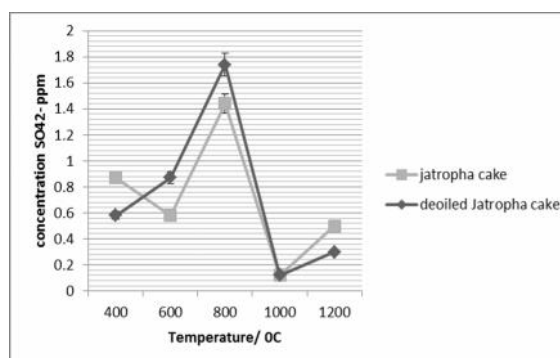
Figure 2: Effect of temperature on the amount of SO 2 produced during combustion
