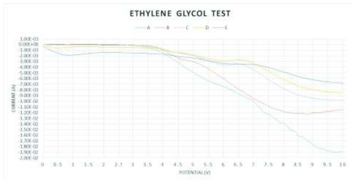
Fig. 3. Electrochemical response of ethylene glycol at the \text{TiO}_2 nanotube electrode
