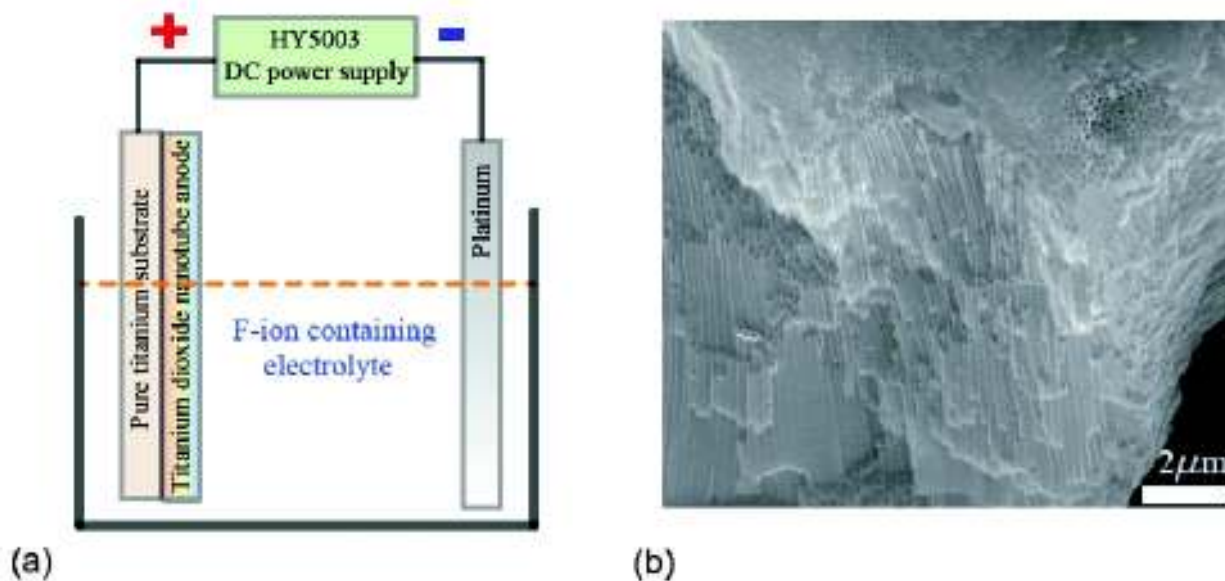
Fig. 1. Schematic of the electrochemical cell for making TiO 2 nanotubes and the image of the nanotube: (a) a sketch of the cell, (b) the image of TiO 2 nanotubes
