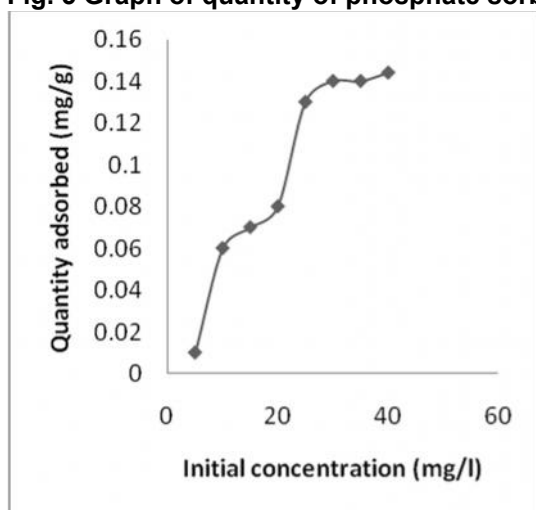
Fig. 6 Graph of quantity of phosphate sorbed by Malete (treated) soil
