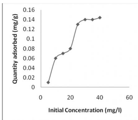
Fig. 5 Graph of quantity of phosphate sorbed by Malete (untreated) soil
