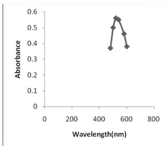
Fig. 1 Graph of absorbance versus wavelength
