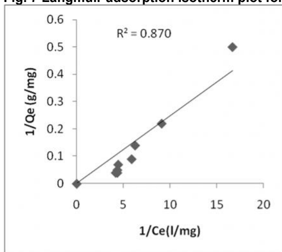
Fig. 8 Langmuir adsorption isotherm plot for Malete soil
