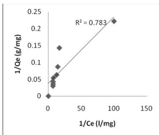
Fig. 7 Langmuir adsorption isotherm plot for Elemere soil
