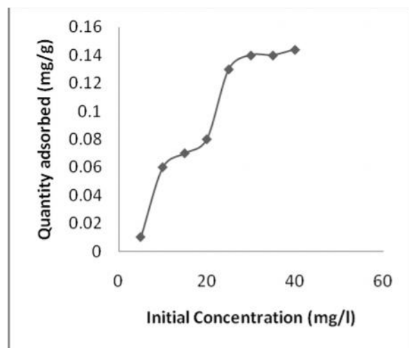
Fig. 4 Graph of quantity of phosphate sorbed by Elemere (treated) soil
