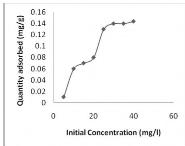
Fig. 3 Graph of quantity of phosphate sorbed by Elemere (untreated) soil
