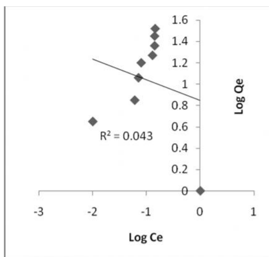
Fig. 9 Freundlich isotherm plot for Elemere Soil
