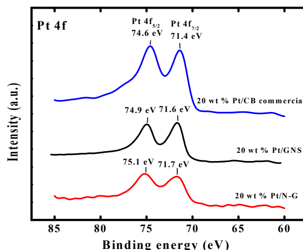
240 Fig. 3. XPS spectra for 20 wt % Pt/GNS, Pt/N-G, and Pt/CB commercial catalyst
