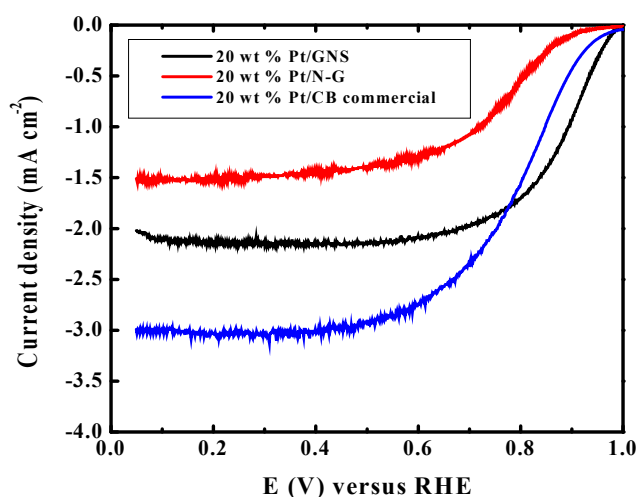
Fig. 1. RRDE polarization curves of 20 wt % Pt/GNS, Pt/N-G, and Pt/CB commercial catalyst in \text{O}_2 -saturated 0.1 M \text{HClO}_4 solution. Scan rate is 10 \text{ mVs}^{-1} . For all the RRDE measurements, the Pt loading of catalysts are 4 \mu\text{g} for 20 wt % Pt/GNS, Pt/N-G, and Pt/CB commercial catalyst, respectively
