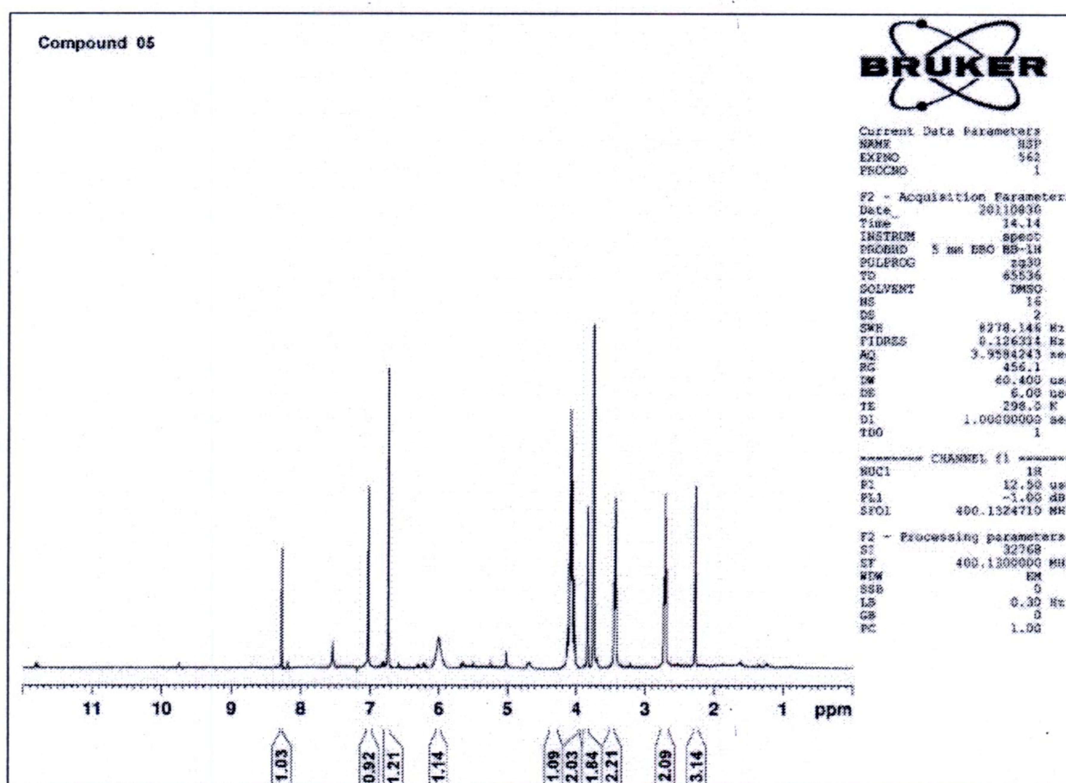
Figure 3: ^1\text{H} -NMR of compound 5a
