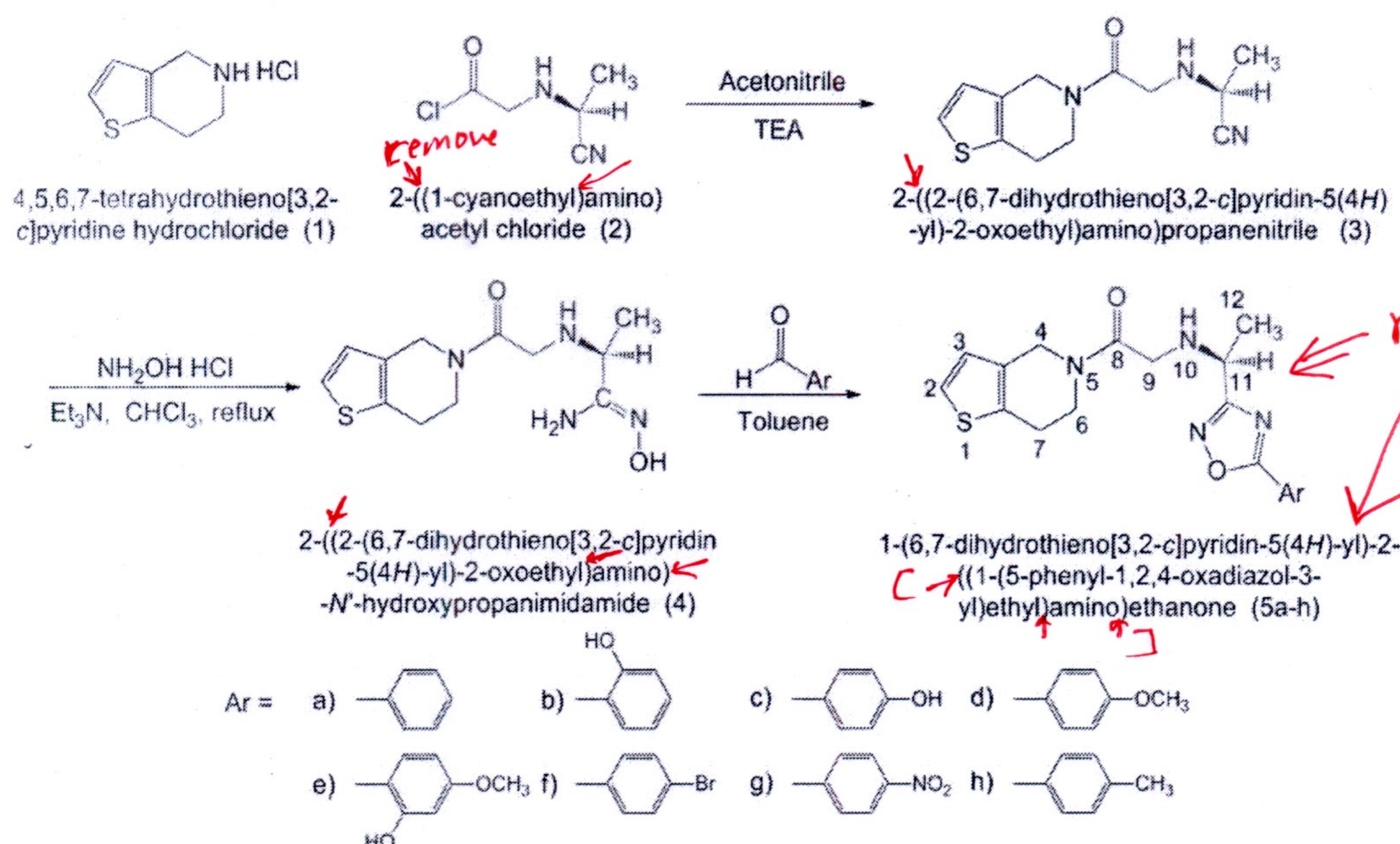
Figure 1: Synthesis of chiral 1,2,4-oxadiazoles 5a-h
