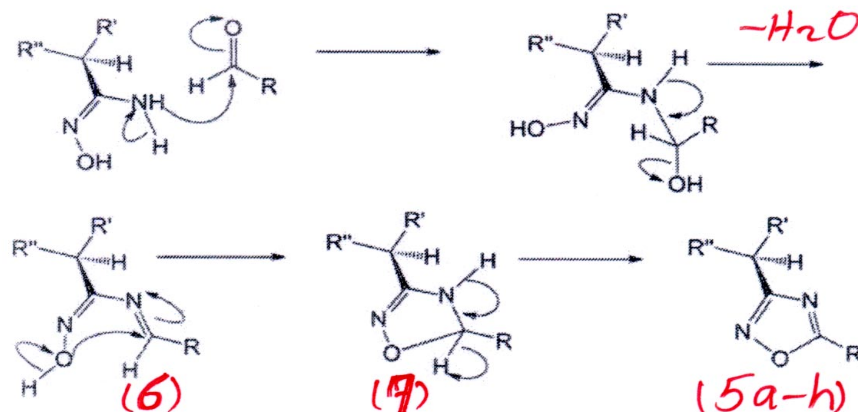
Figure 2: Proposed mechanism for the synthesis of 1,2,4-oxadiazole
